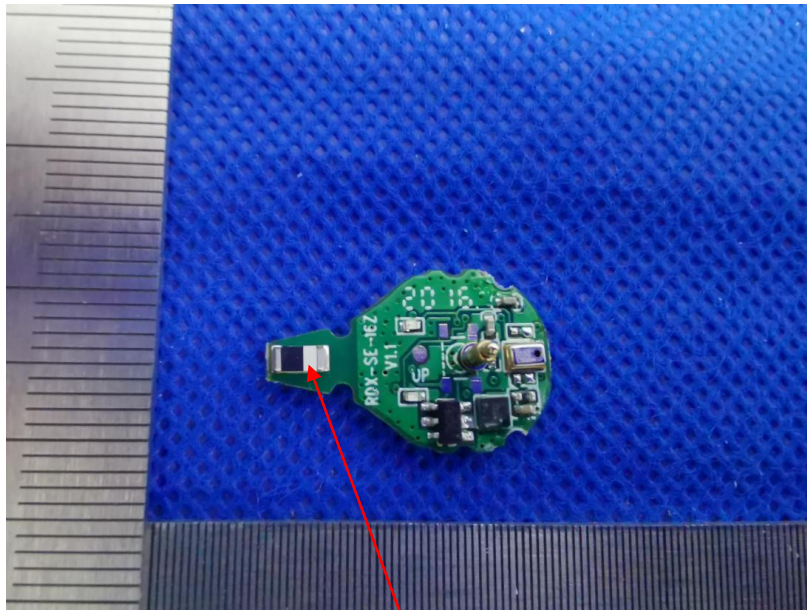
Chip Antenna
