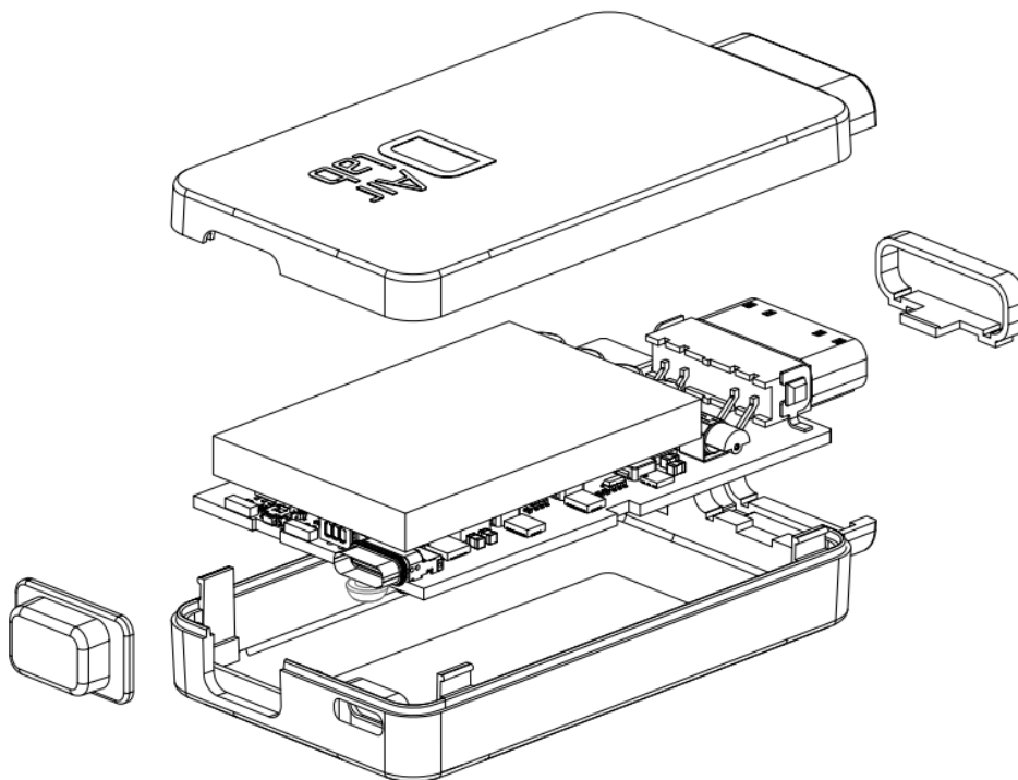
Figure 1: electronic control unit
