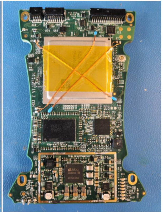
Wireless Module (Wifi and Bluetooth)
