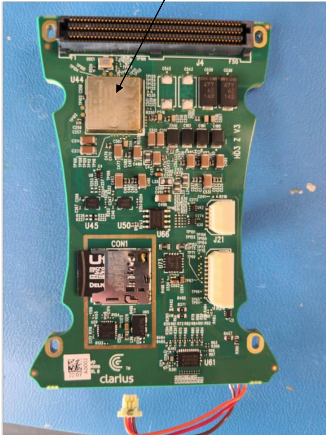
Wireless Module (Wifi and Bluetooth)
