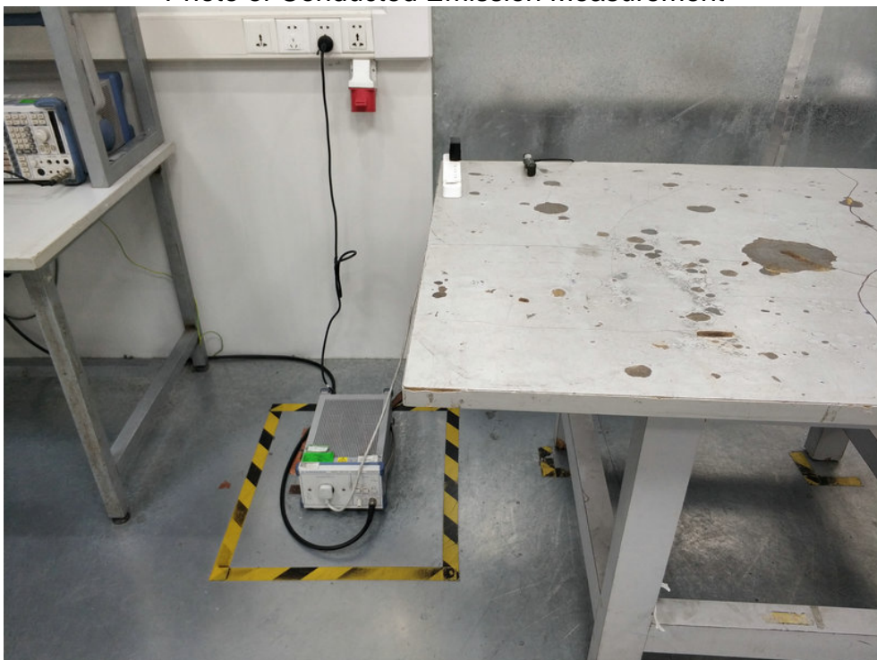
FCC ID: 2AWLM-MUJAMINI Photo of Conducted Emission Measurement
