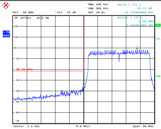
802.11ax hew40_Chain 0_Lowest Band edge
