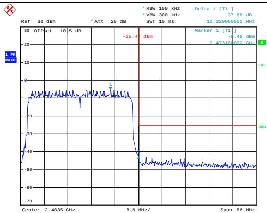
802.11ax hew40_Chain 0_Highest Band edge
