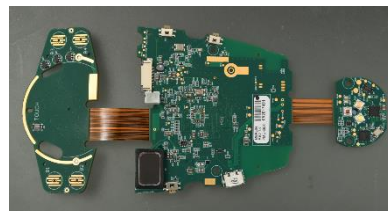
Main Board Bottom
