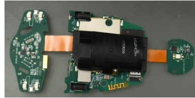
Antenna Top View
