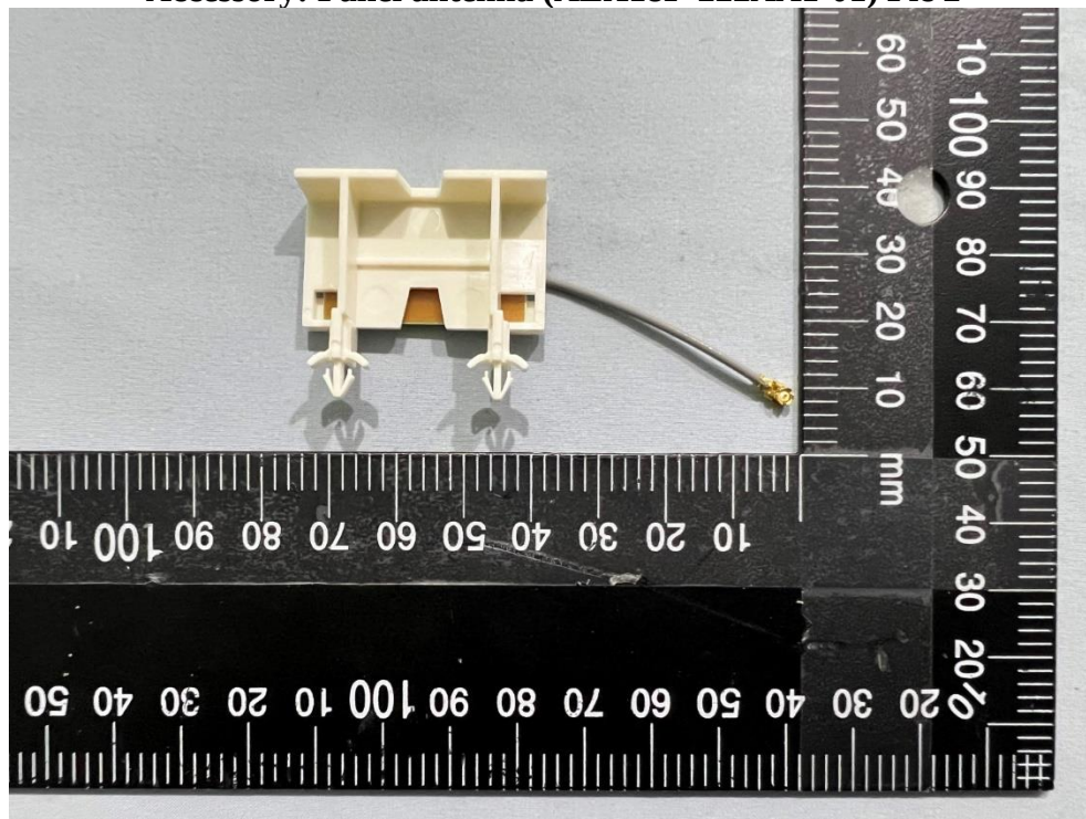
Accessory: Panel antenna (ALX18P-222AA1-01) Pic 2
