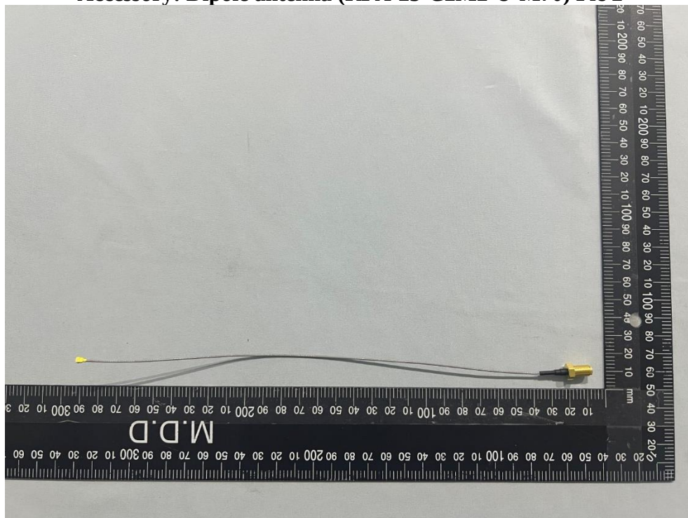
Accessory: Dipole antenna (RFA-25-C2M2-U-M70) Pic 2
