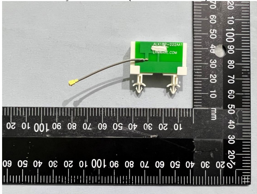
Accessory: Panel antenna (ALX18P-222AA1-01) Pic 1
