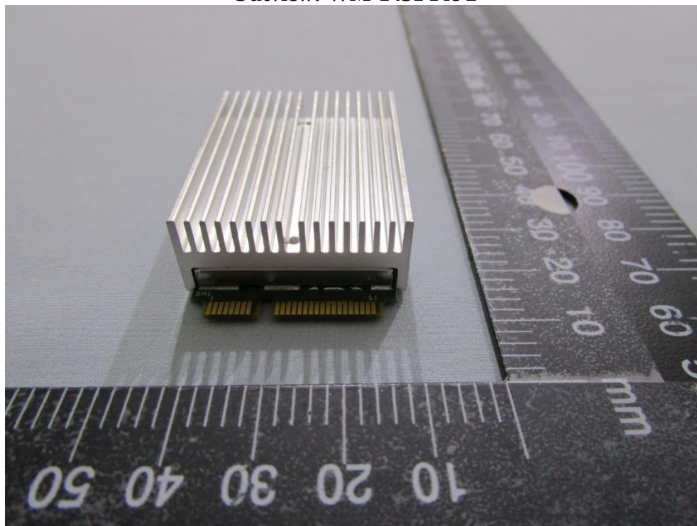
Outview: WM-1431 Pic 2
