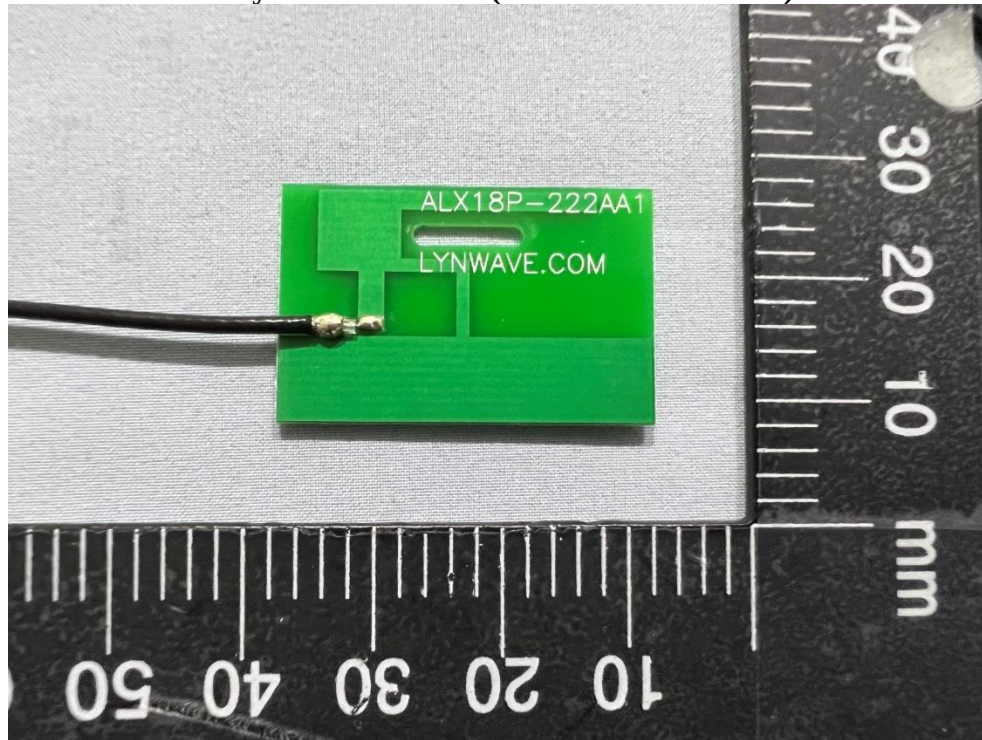
Accessory: Panel antenna (ALX18P-222AA1-00) Pic 3
