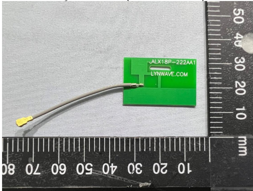
Accessory: Panel antenna (ALX18P-222AA1-01) Pic 3
