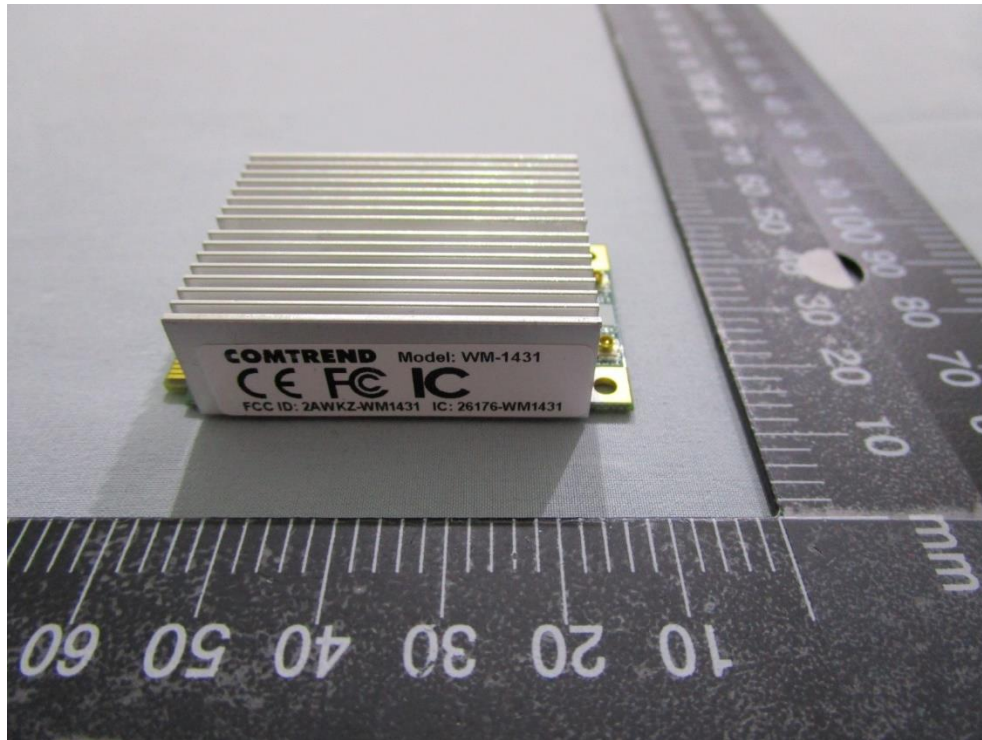
Outview: WM-1431 Pic 3
