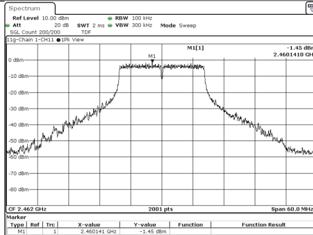
802.11g, CH11, Chain 1, Conducted Emission
