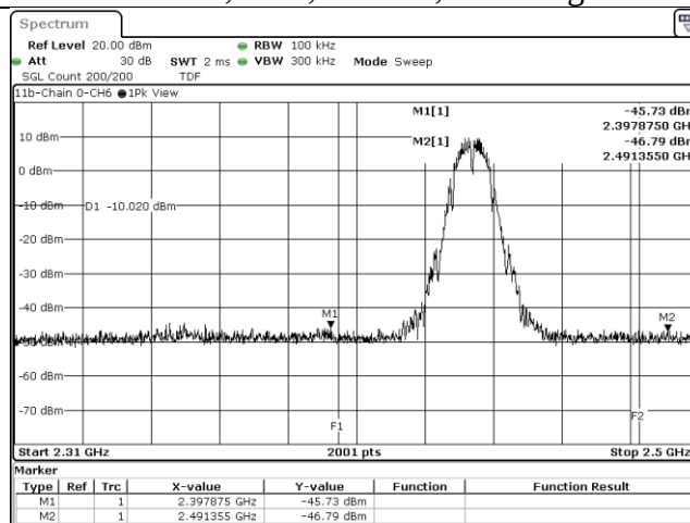
802.11b, CH6, Chain 0, Band edge
