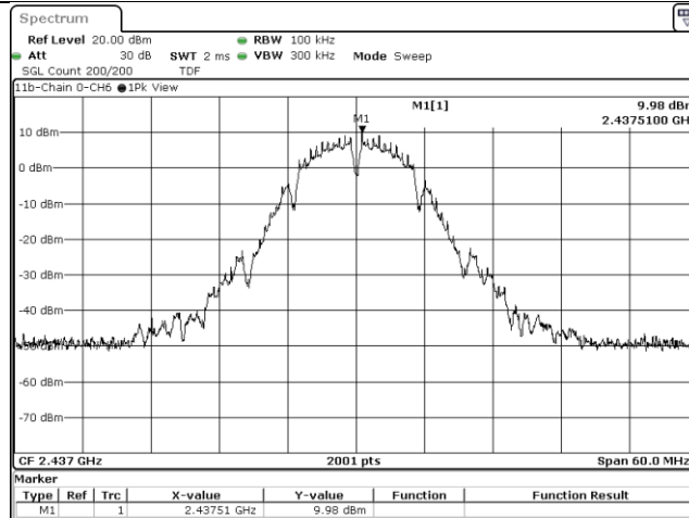
802.11b, CH6, Chain 0, Conducted Emission
