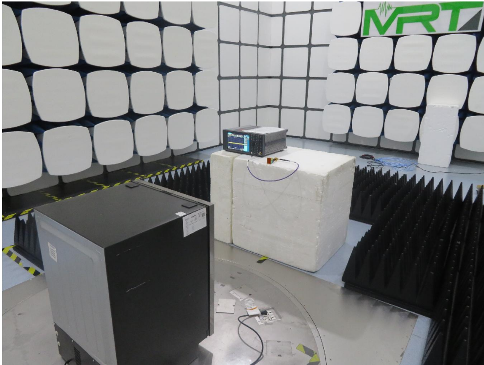
Description: Radiated Emission Test Setup for 50GHz ~ 75GHz
