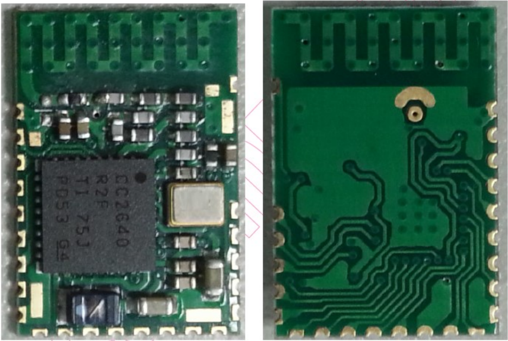
Figure 12 Internal View (RF Module, Front & Back View)
