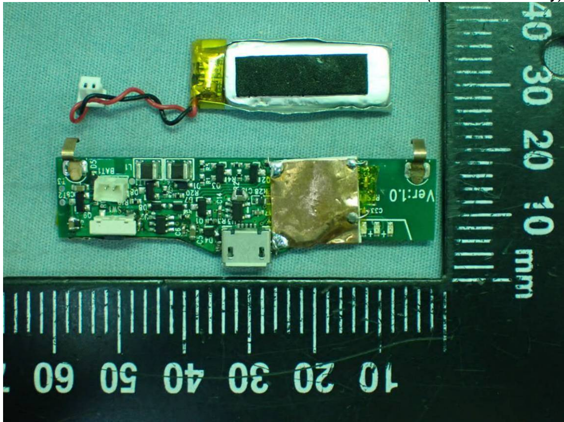
Figure 9 Internal View (Removed Battery)
