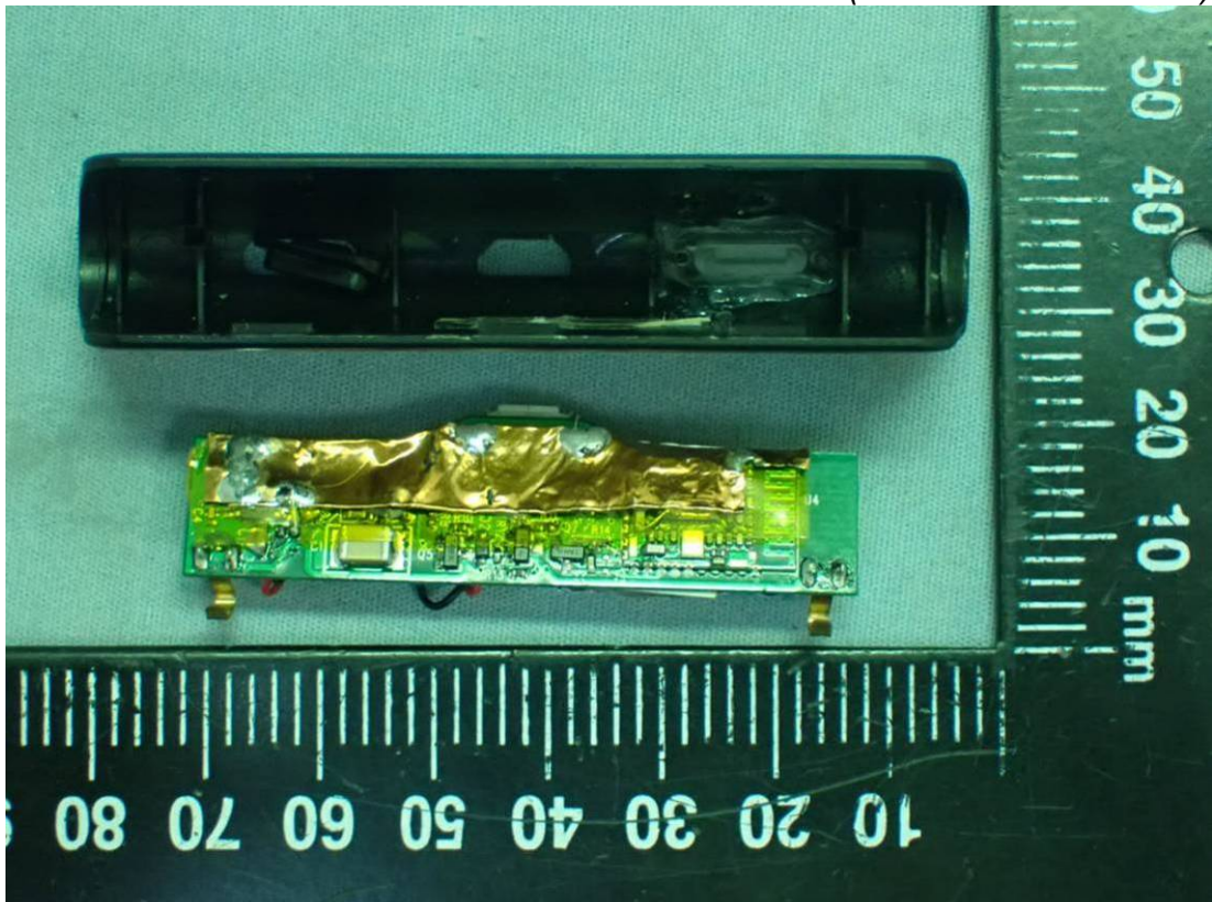
Figure 8 Internal View (Removed Main Board)
