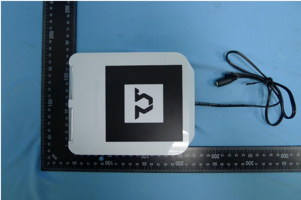
(7) EUT Photo
