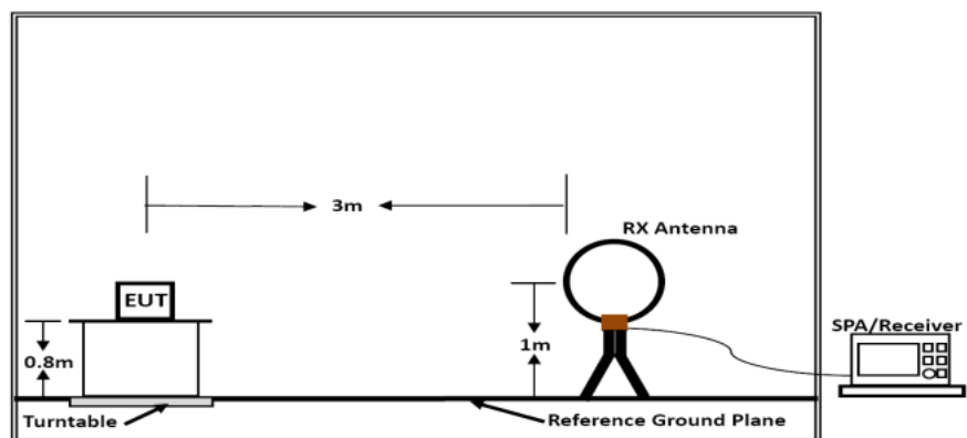
Below 30MHz
