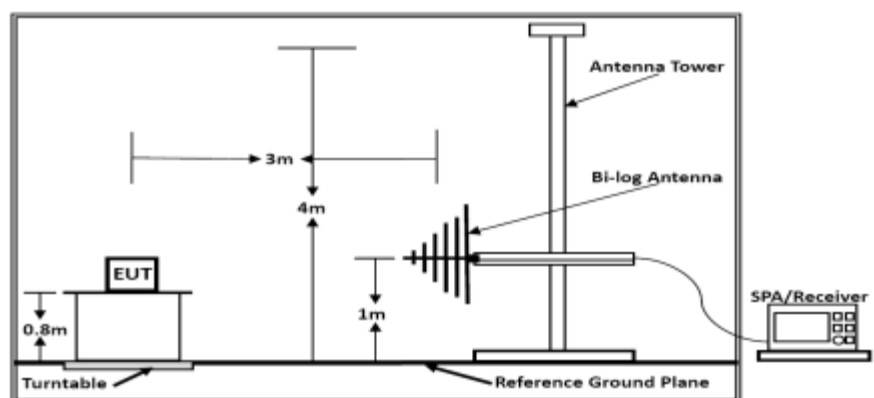
Below 1GHz
