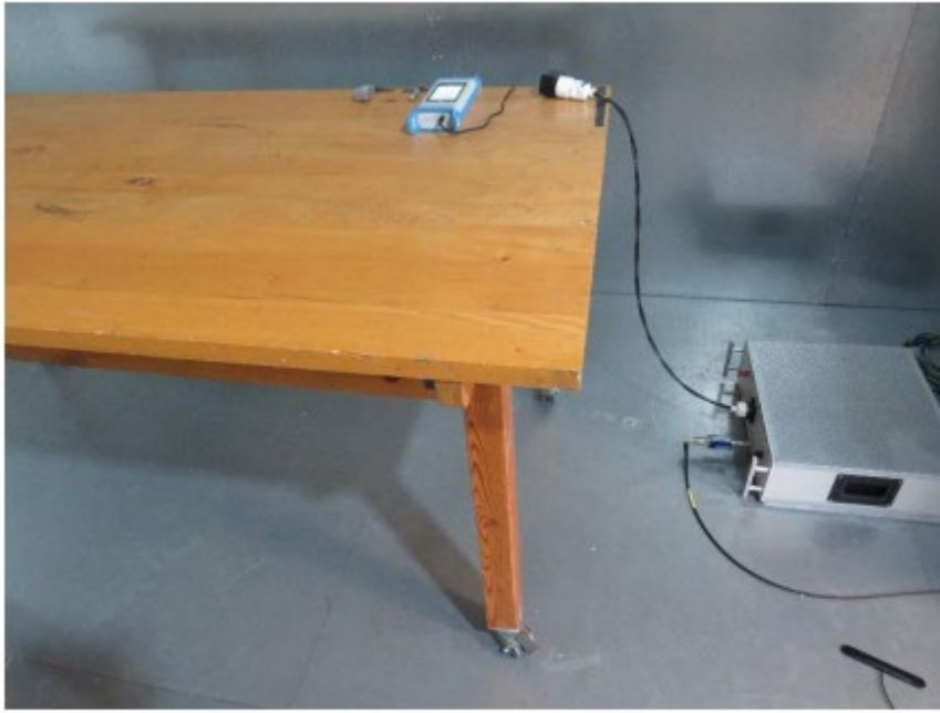
Setup for measurements 150 kHz – 30 MHz
