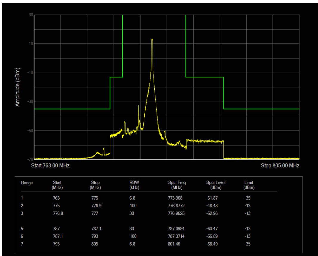
LTE Band13 QAM16 BW=5MHz Channel=23205 RB Size=1 Position=#Max
