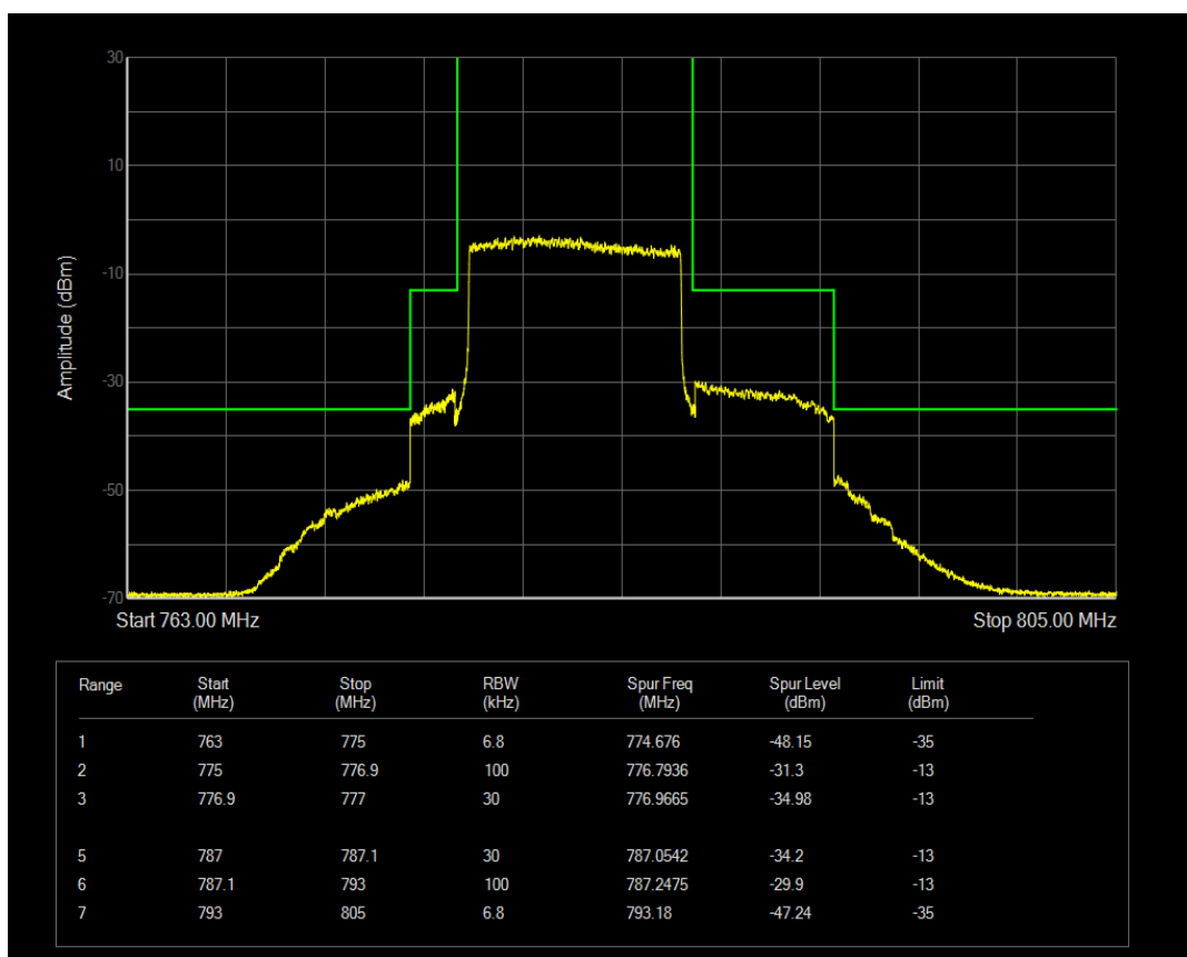
LTE Band13 QAM16 BW=10MHz Channel=23230 RB Size=1 Position=#Max
