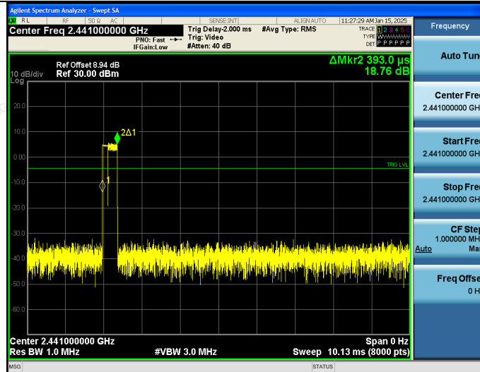
2-DH1
