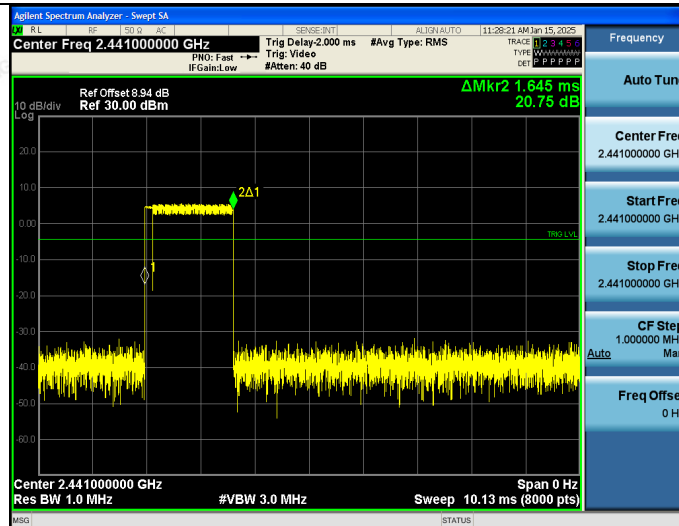
2-DH3
