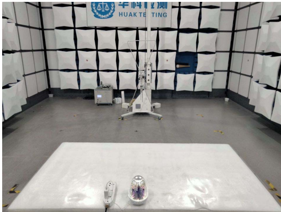
Model: YS-BS0176 Radiated Emissions
