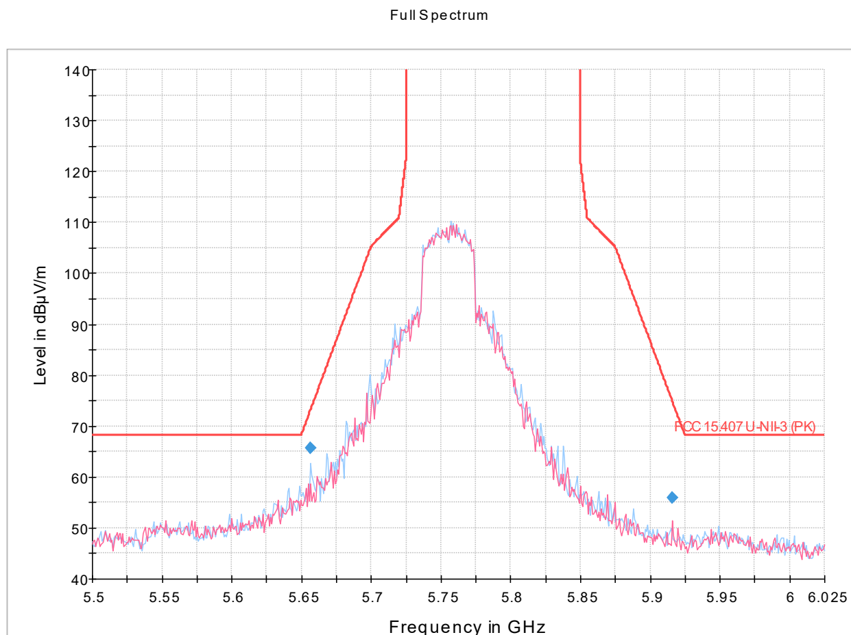
Figure 8.10-65: Radiated emissions spectral plot (5.5 GHz - 6.025 GHz), 5755 MHz operation
