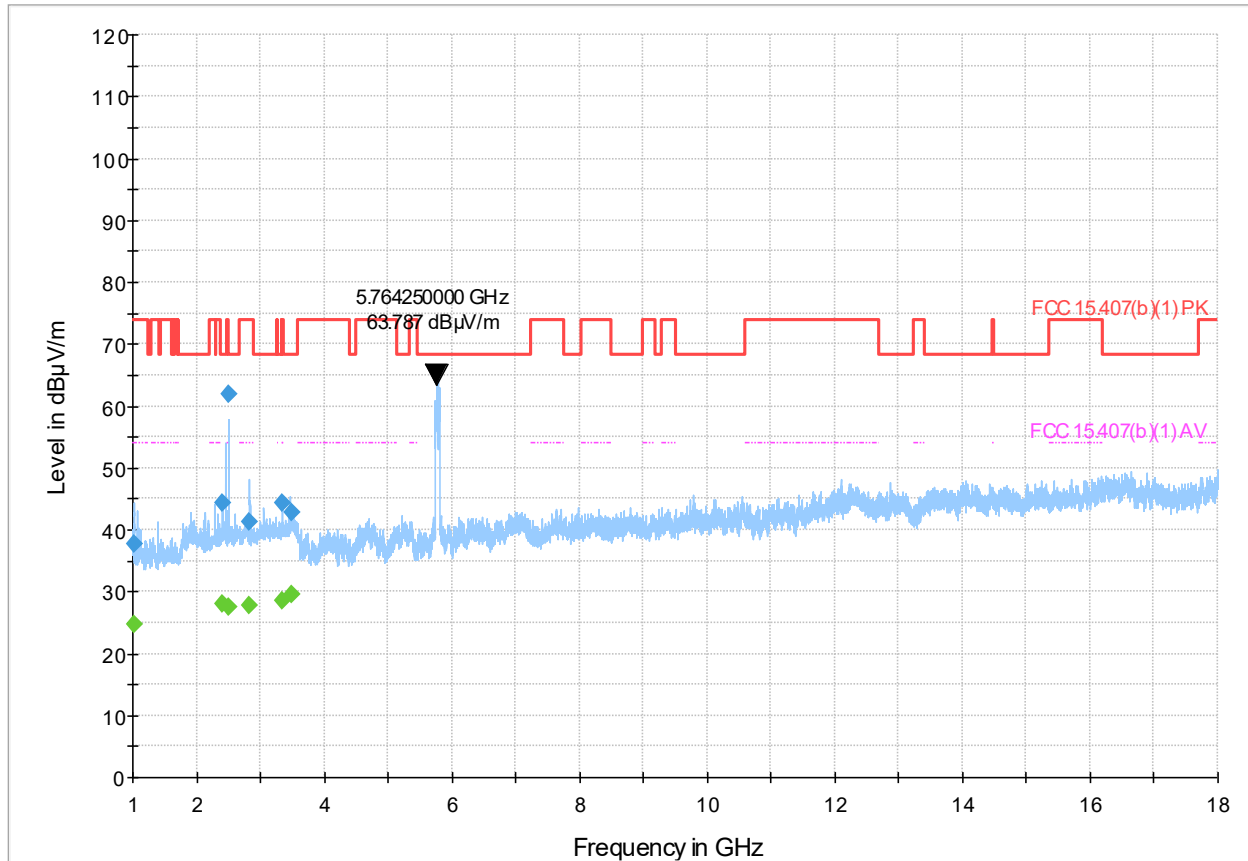
Figure 8.10-67: Radiated emissions spectral plot (1 GHz - 18 GHz), 5775 MHz operation
