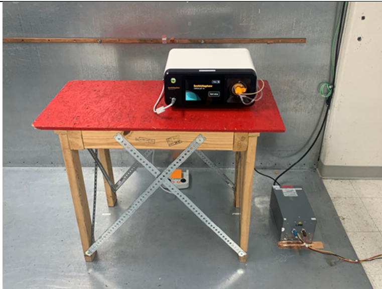
AC Line Conducted Emissions
