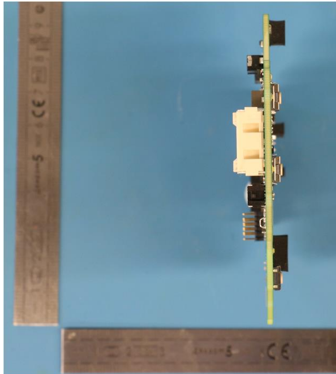
16- Main Board Assembly, left side view
