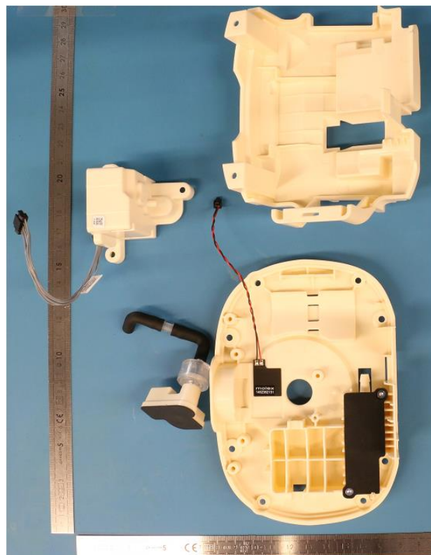
44- Bottom enclosure with internal assemblies and Manifold assembly
