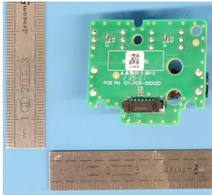
28- Manifold Board Assembly, left side view
