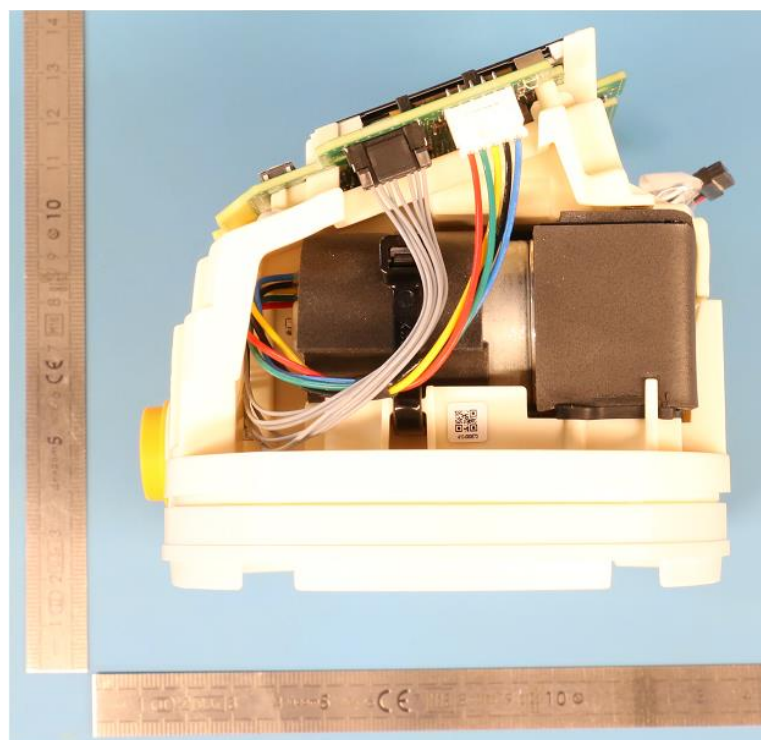
8- Internal assembly right side view with Pump and Cables interfaces.
