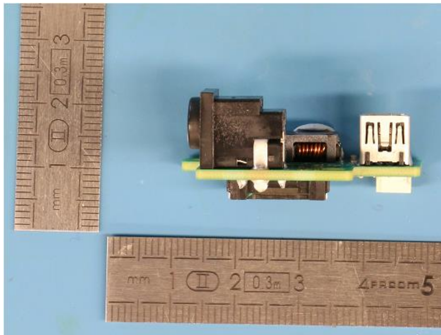
25- Rear Trim Board Assembly, top view
