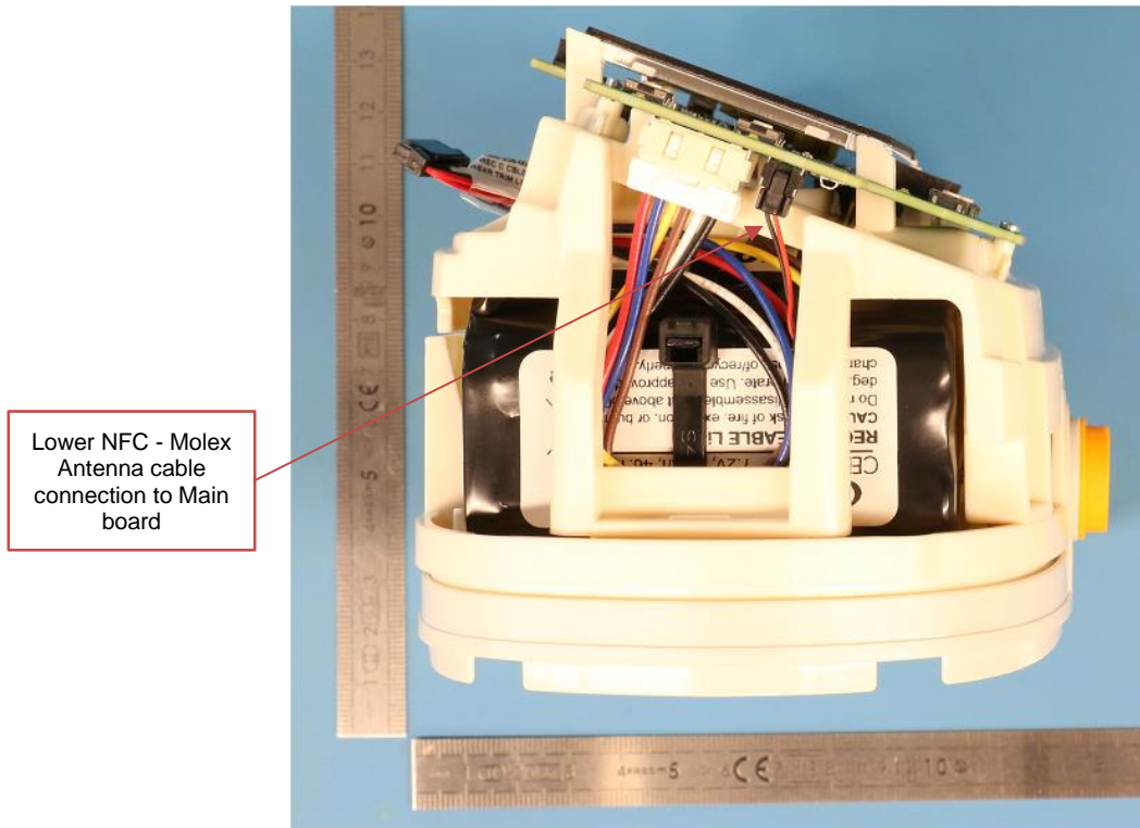
8- Internal assembly right side view with Pump and Cables interfaces.
