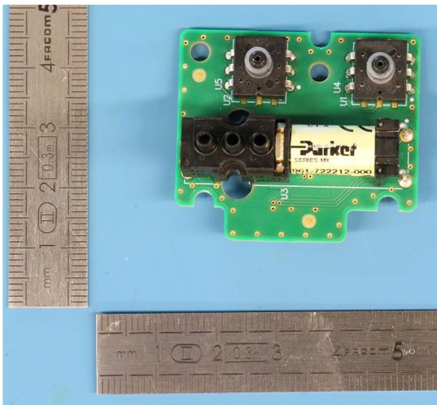
26- Manifold Board Assembly, front view
