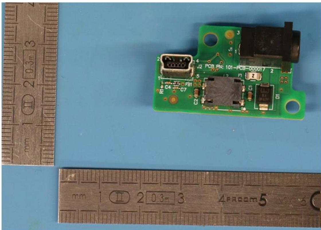
20- Rear Trim Board Assembly, front view
