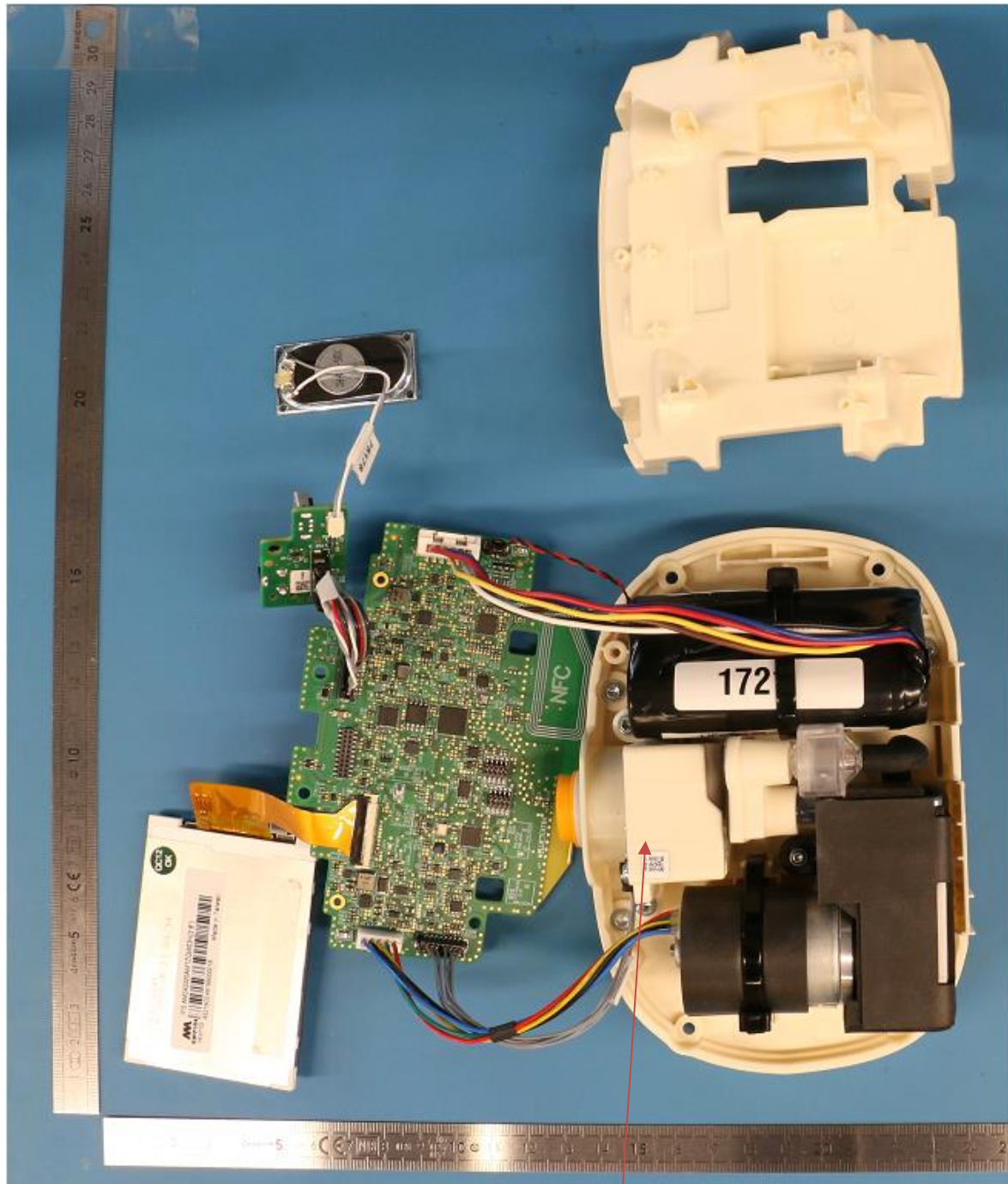
Manifold Assembly with Manifold Board inside. Connected to Main board via a cable assembly
