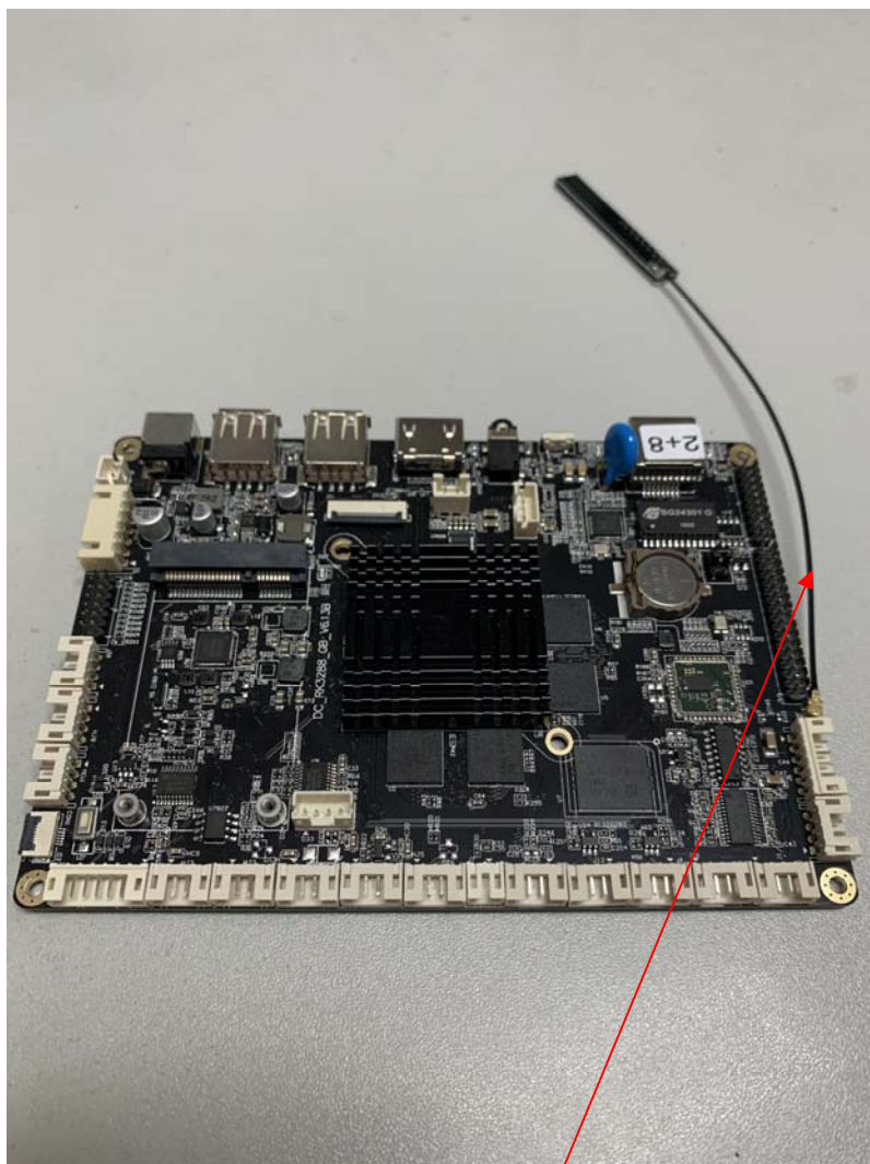
WIFI & BT Antenna
