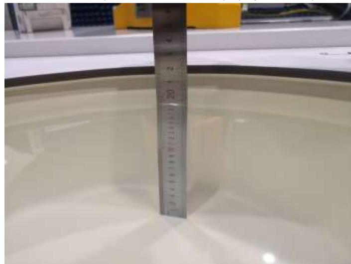
Fig. 9.2 Photo of Liquid Height for Body SAR of Twin Phantom (5000MHz~5800MHz) (depth>15cm)
