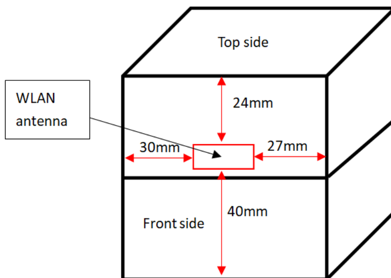
Fig.12.1 EUT Antenna Locations
