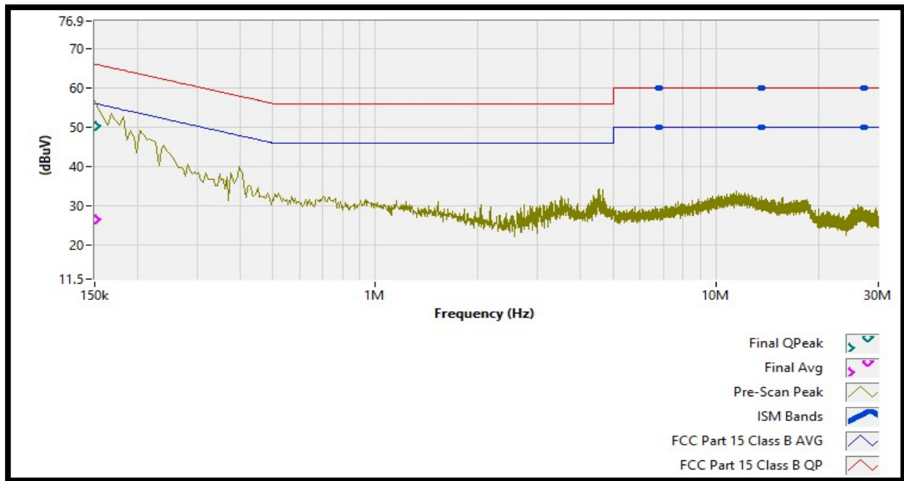
Plot 4 – Conducted Emissions – Neutral Side (Idle Mode)
