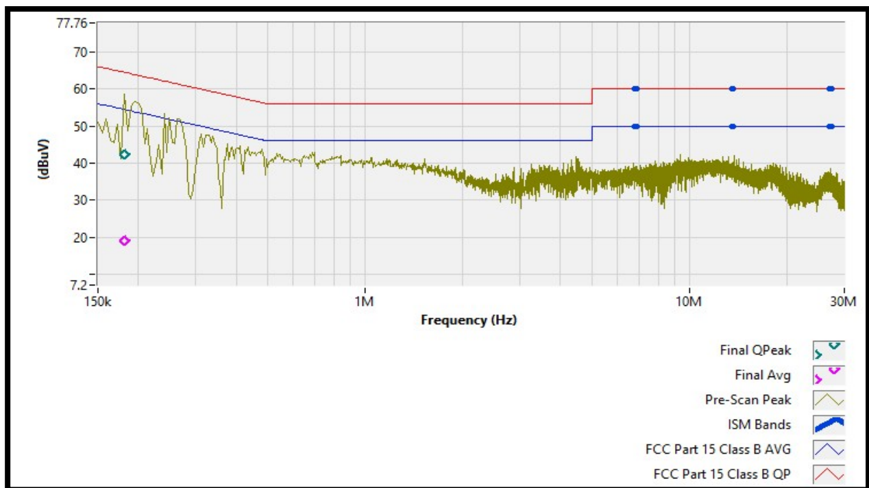
Plot 3 – Conducted Emission – Line Side (WPT Mode)
