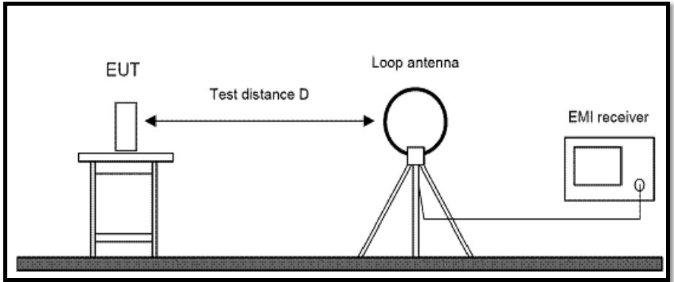
Figure 4. Radiated Emissions Test Setup (9kHz - 30MHz)
