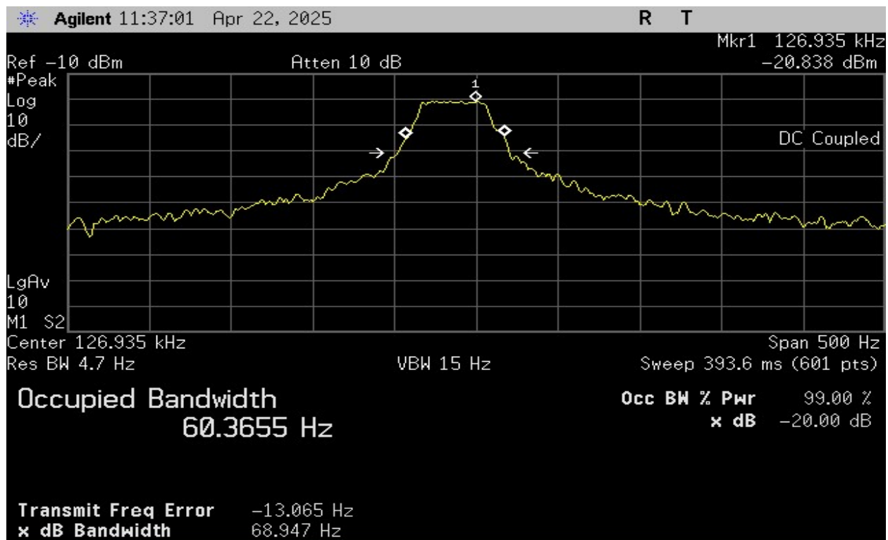
Plot 7 – 20dB BW – WPT Mode
