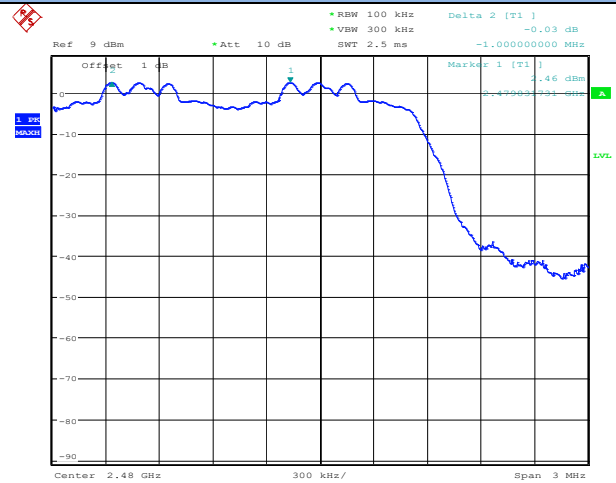
\pi/4 -DQPSK / High Channel
