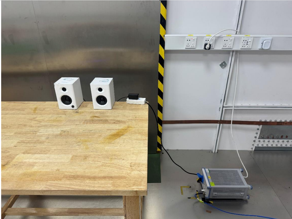
Conducted Output Power
