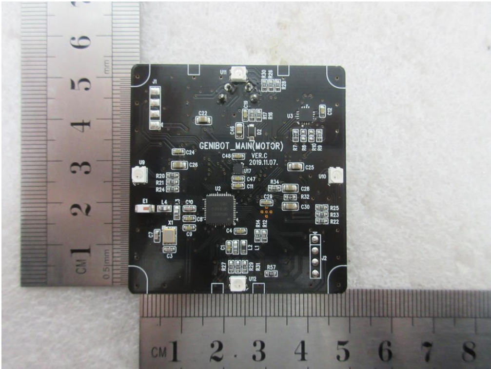
Main board_Front
