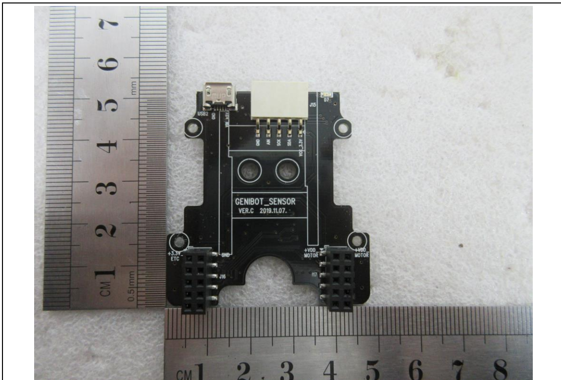
Sensor board_Front
