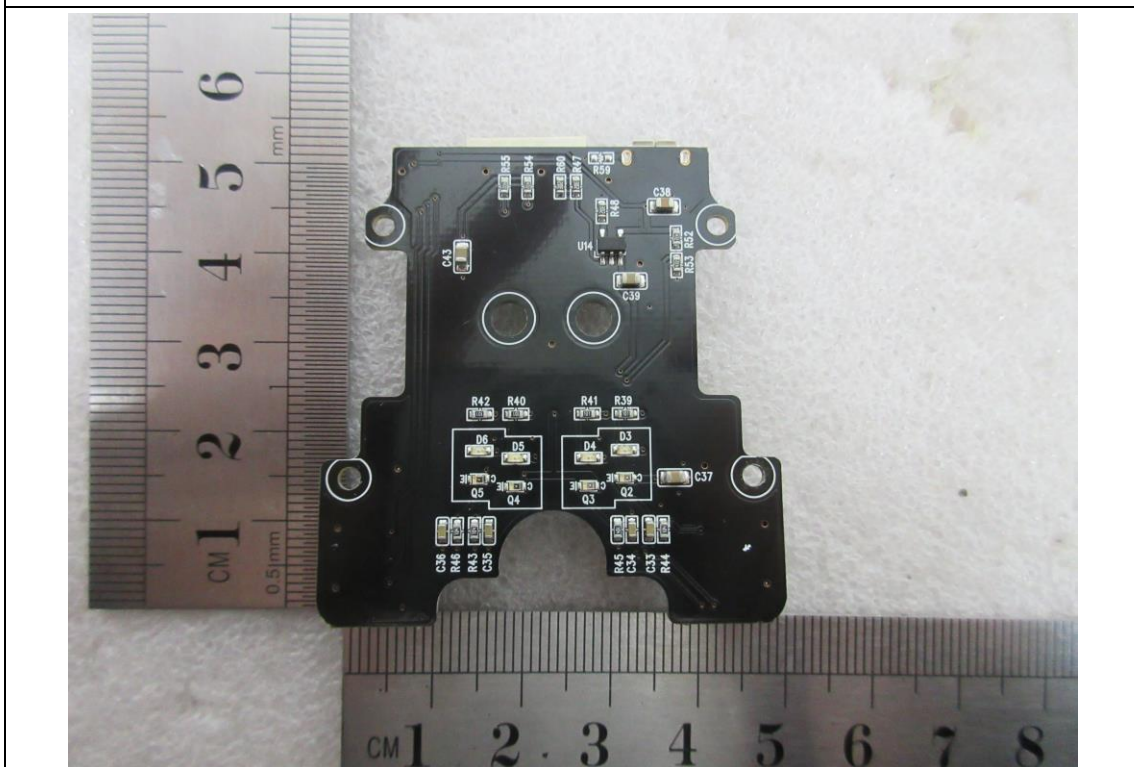
Sensor board_Rear
