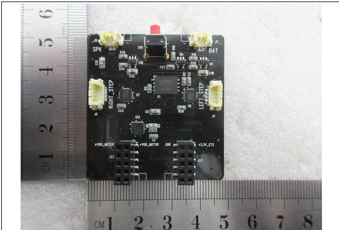
Main board_Rear
