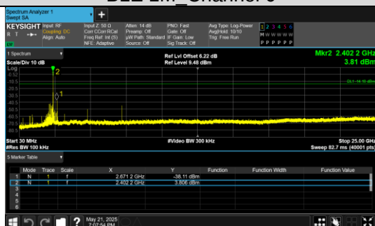
30.0 MHz - 25000.0 MHz BLE 1M Channel 0
