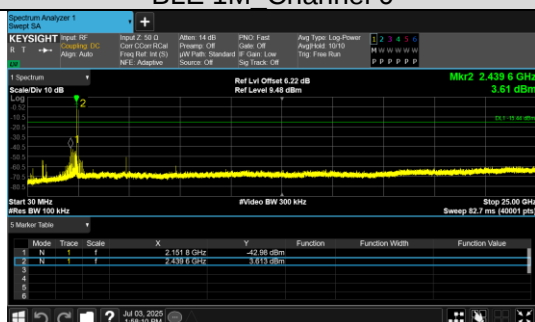
30.0 MHz - 25000.0 MHz BLE 1M Channel 19
