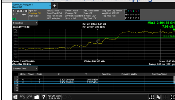
Out Of Band Emission(Left) 8DPSK_3-DH5_Channel Hopping
