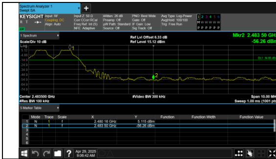
Out Of Band Emission(Right) GFSK_DH5_Channel Hopping
