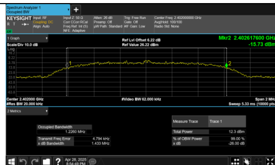
8DPSK_3-DH5_Channel 0
