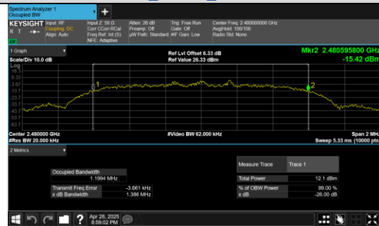
8DPSK_3-DH5_Channel 78
