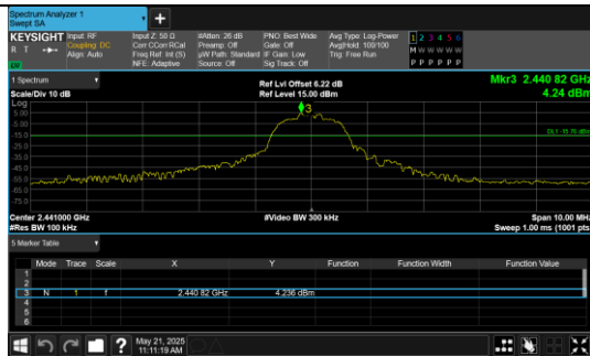
Out Of Band Emission 8DPSK 3-DH5 Channel 39
