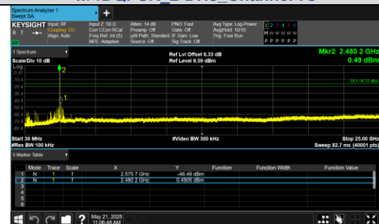
30.0 MHz - 25000.0 MHz π/4DQPSK 2-DH5 Channel 78
