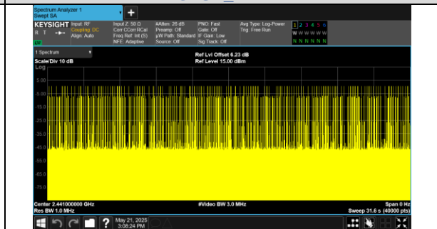
Number of Pulses in 31.6 seconds GFSK_DH3
