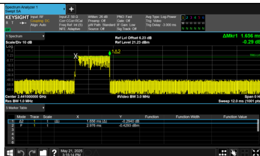
Pulse Width 8DPSK 3-DH3
