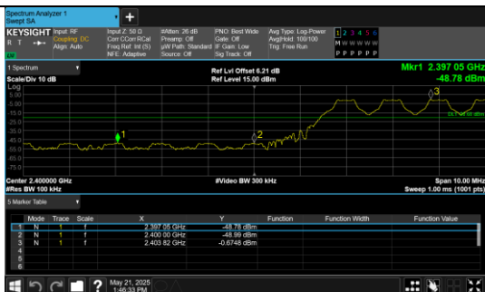
Out Of Band Emission(Left) GFSK DH5 Channel Hopping
