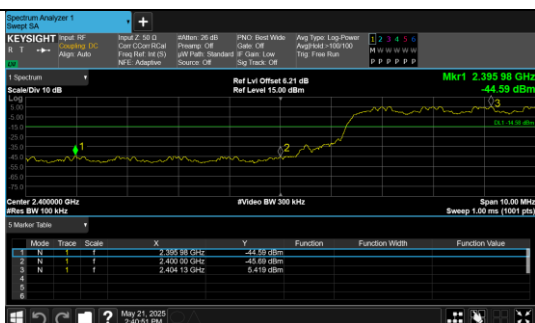
Out Of Band Emission(Left) 8DPSK 3-DH5 Channel Hopping
