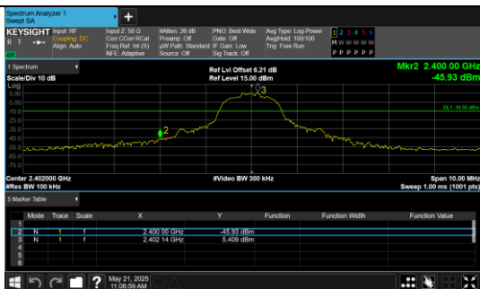
Out Of Band Emission 8DPSK 3-DH5 Channel 0
