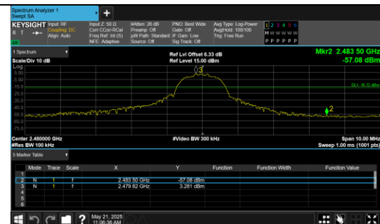
Out Of Band Emission π/4DQPSK 2-DH5 Channel 78
