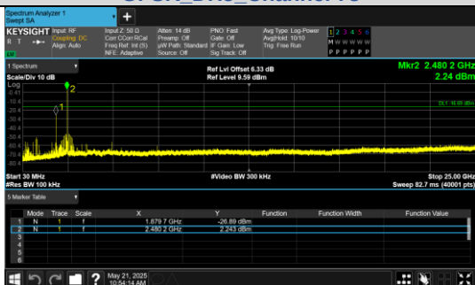
30.0 MHz - 25000.0 MHz GFSK DH5 Channel 78
