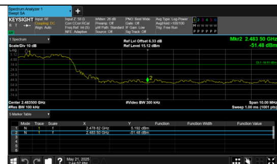
Out Of Band Emission(Right) 8DPSK 3-DH5 Channel Hopping
