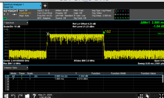
Pulse Width 8DPSK 3-DH5
