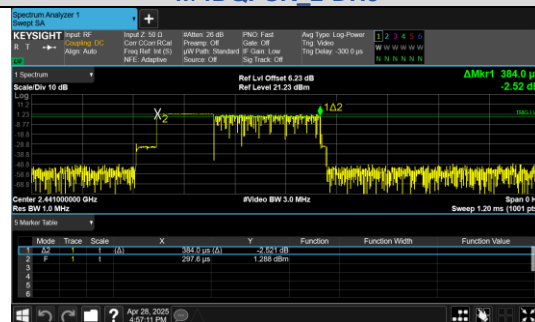
Pulse Width 8DPSK 3-DH1
