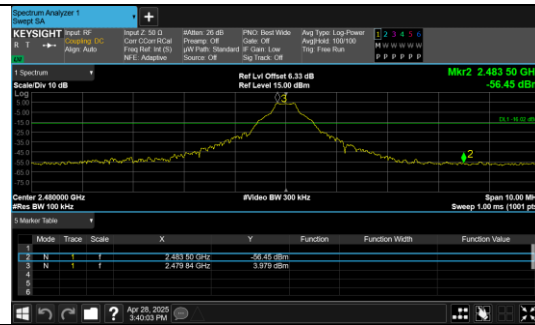
Out Of Band Emission GFSK_DH5_Channel 78
