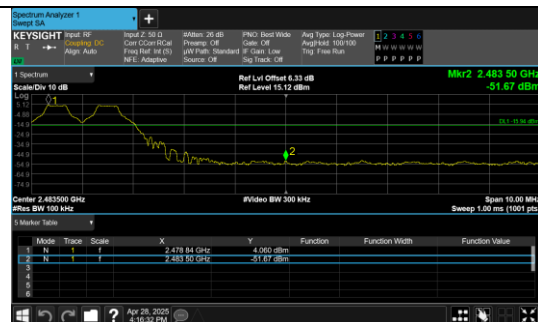
Out Of Band Emission(Right) GFSK_DH5_Channel Hopping
