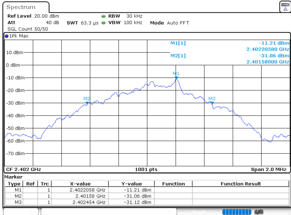
-20 dB BW NVNT 1-DH5 2402MHz Ant1
