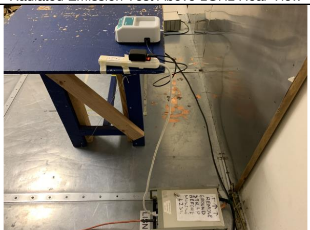
Conducted Emission Test Side View
