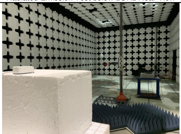
Radiated Emission Test Above 1GHz Rear View
