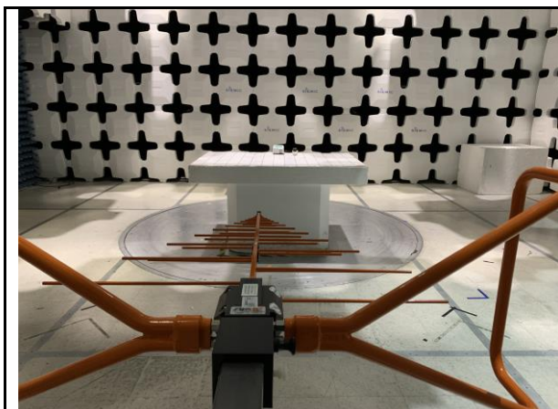
Radiated Emission Test below 1GHz Front View
