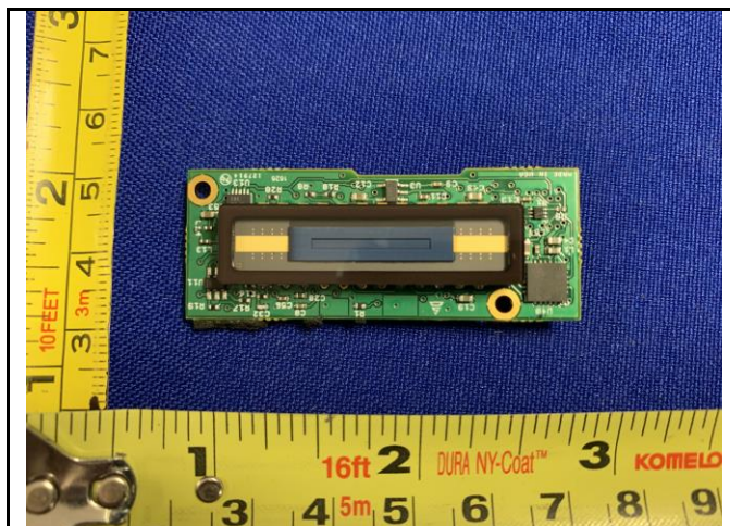
PCB3 Rear View
