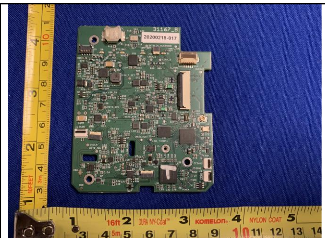
PCB1 Front View
