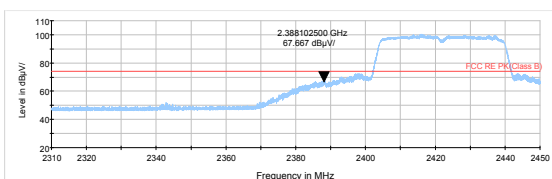
802.11n HT40 -Channel 3 Peak
