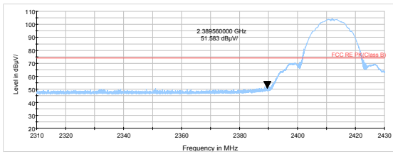
802.11b-Channel 1 Peak
