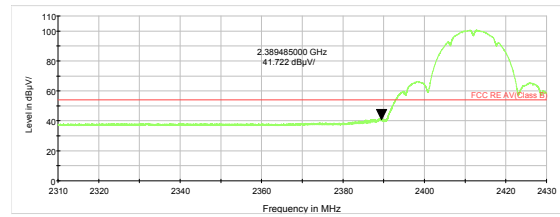
802.11b-Channel 1 Average
