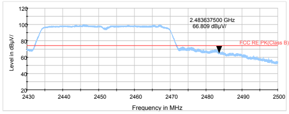
802.11n HT40 -Channel 9 Peak
