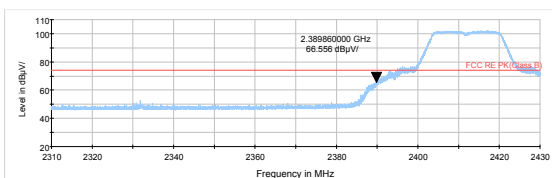
802.11n HT20 -Channel 1 Peak
