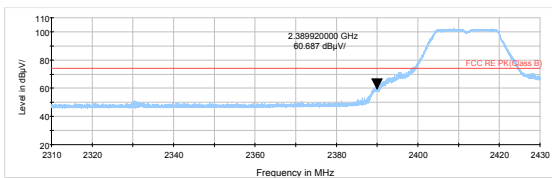
802.11g-Channel 1 Peak
