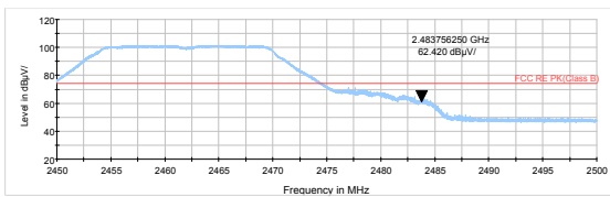
802.11g-Channel 11 Peak
