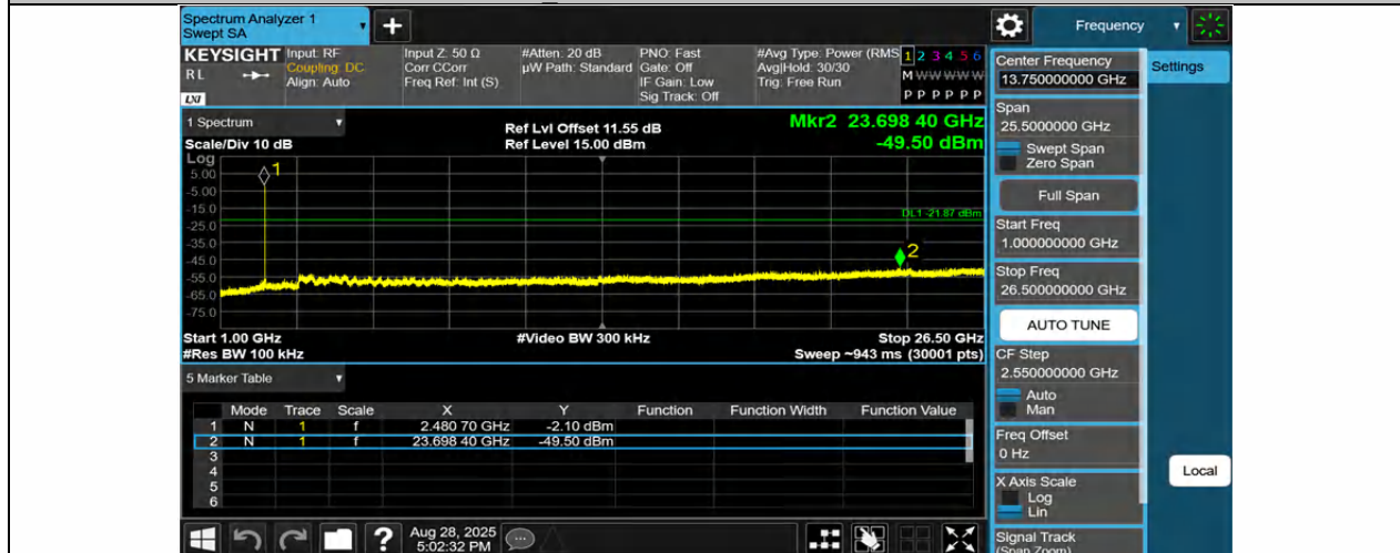
BLE_2M-Ant1-2480-1000~26500-PASS
