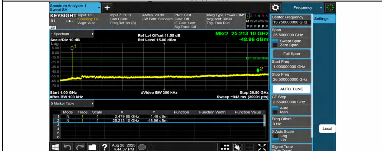
BLE_1M-Ant1-2480-1000~26500-PASS
