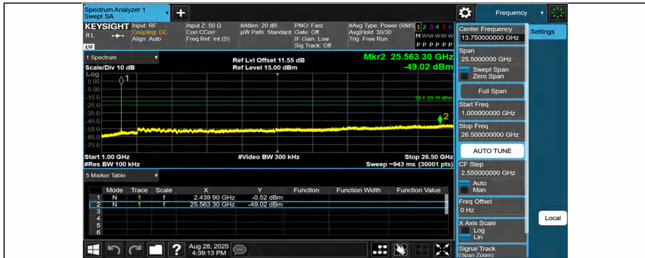
BLE_1M-Ant1-2440-1000~26500-PASS
