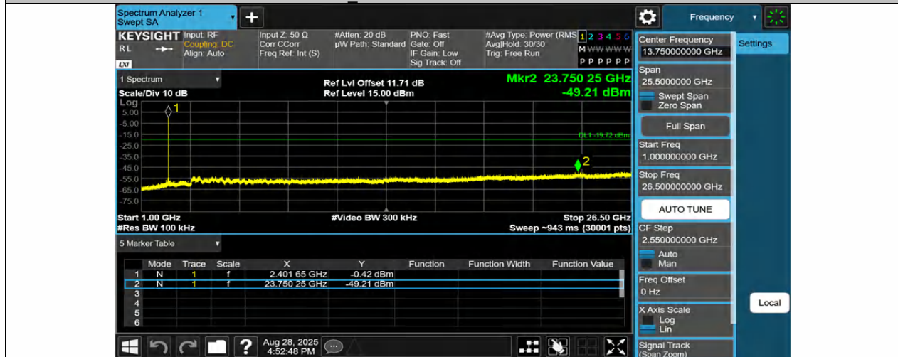
BLE_2M-Ant1-2402-1000~26500-PASS
