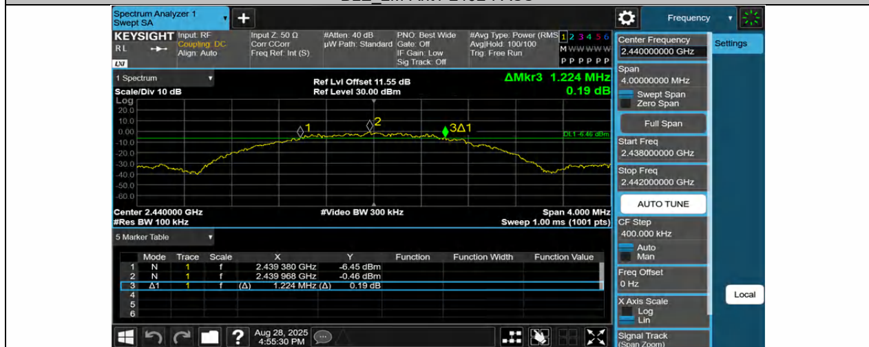
BLE_2M-Ant1-2440-PASS
