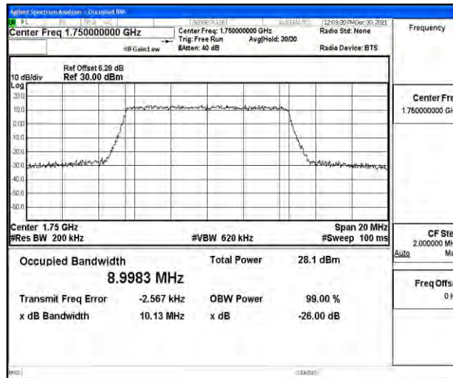
Band4-10MHz-16QAM-20000
