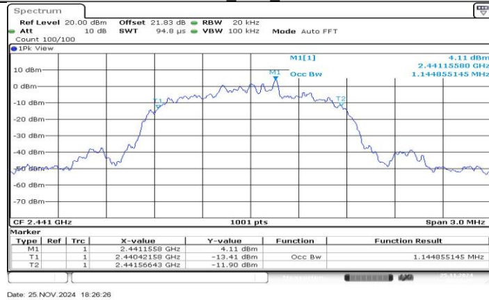
3DH5 Ant1_2441
