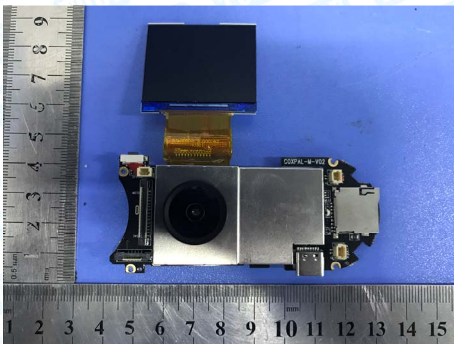
Photo 21 Internal of EUT
