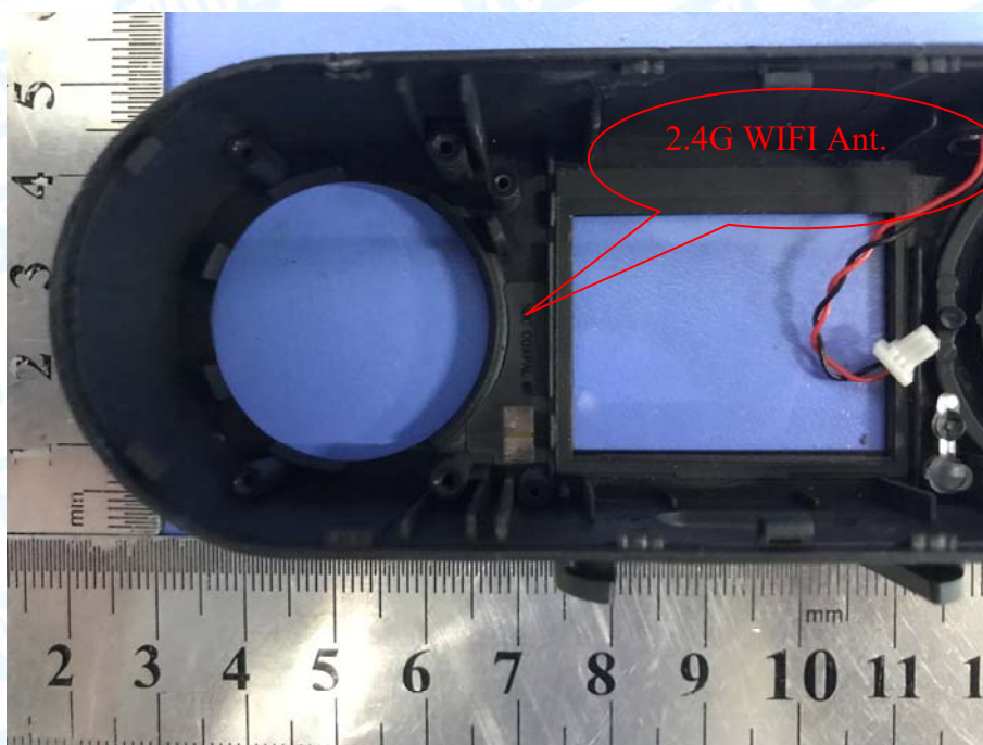
Photo 25 Internal of EUT
