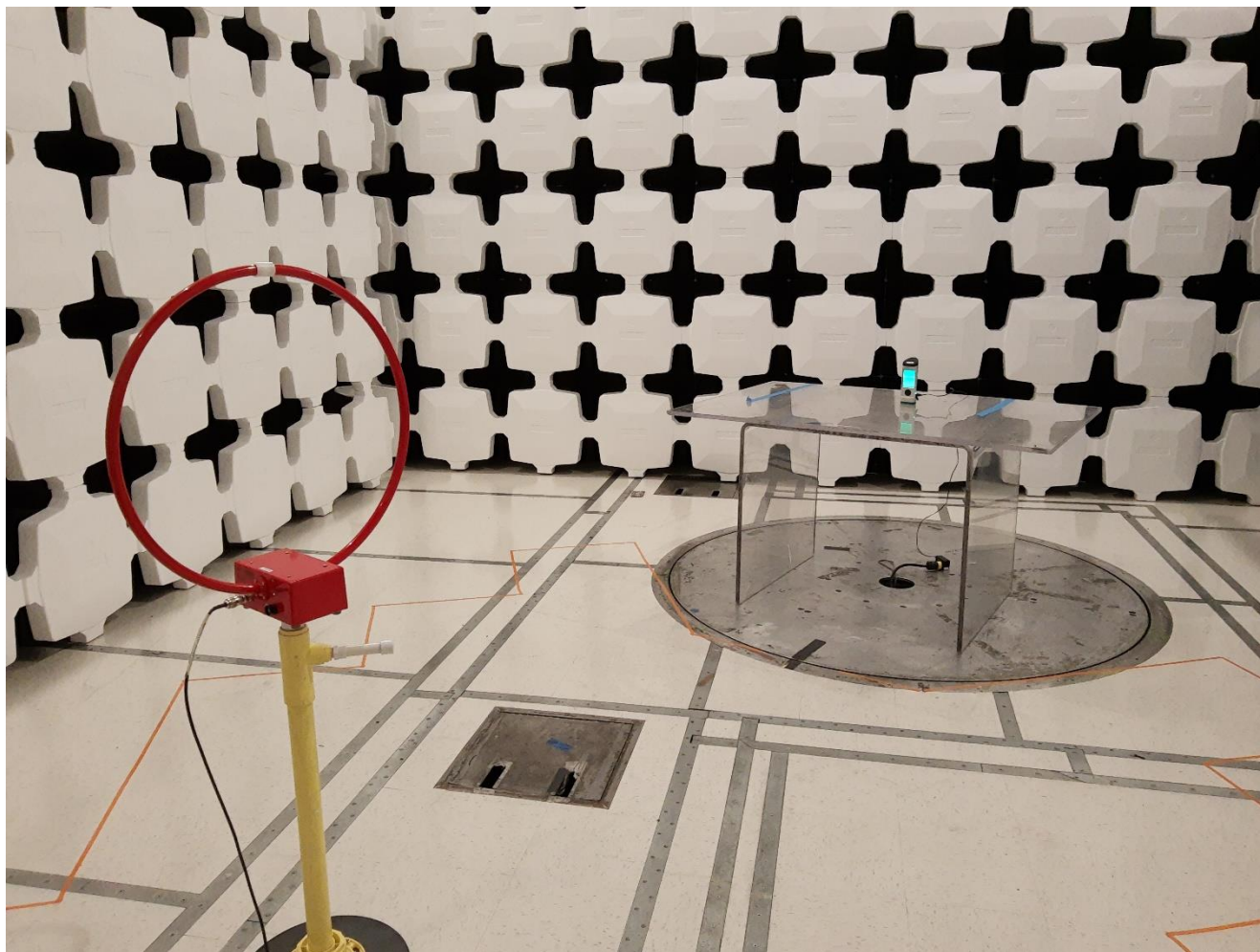
Photograph 2. Radiated Emissions 9kHz - 30 MHz Parallel Test Setup
