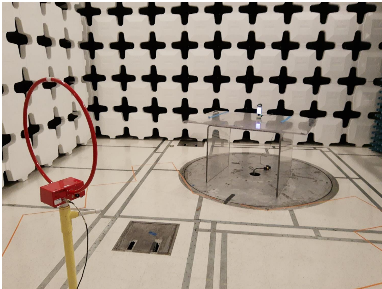
Photograph 1. Radiated Emissions 9kHz - 30 MHz Parallel Test Setup
