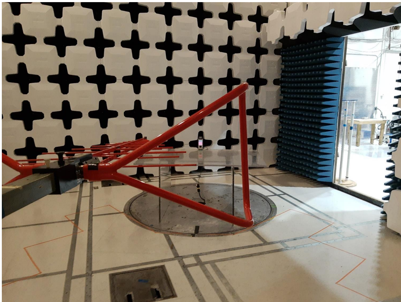
Photograph 3. Radiated Emissions 30-1000 MHz Test Setup
