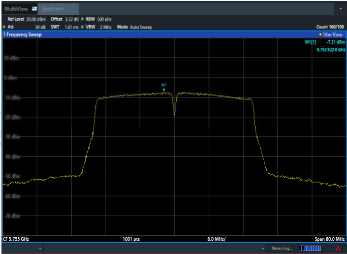
11AC40SISO_Ant2_5755
