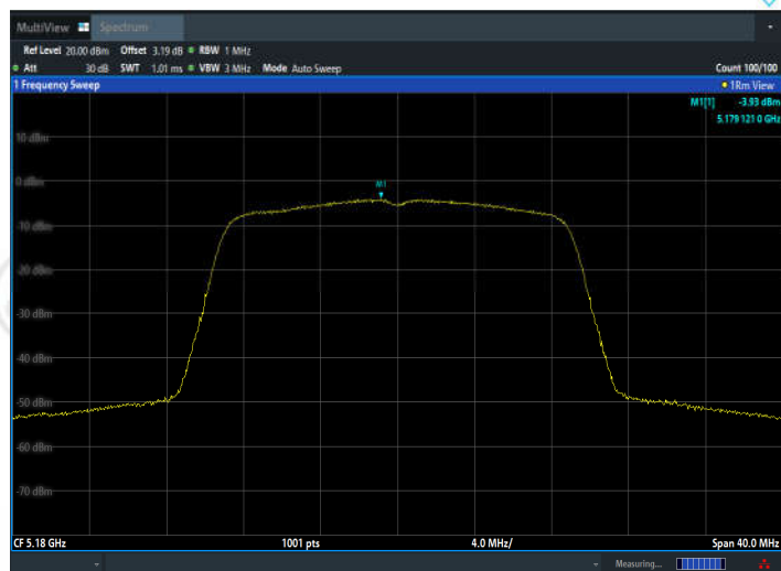
11AC20MIMO Ant2 5180
