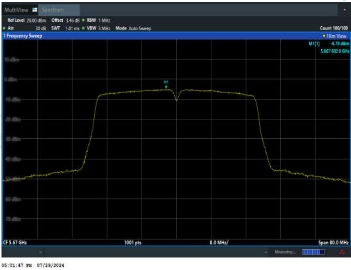
11AC40SISO_Ant2_5670
