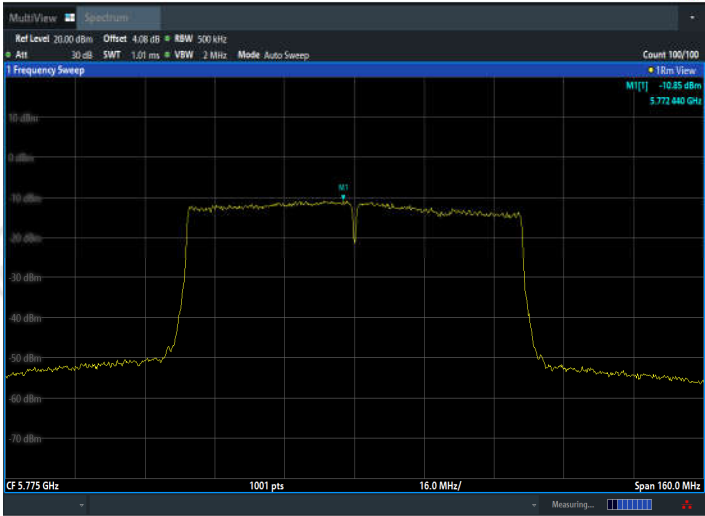
11AC80SISO_Ant2_5775
