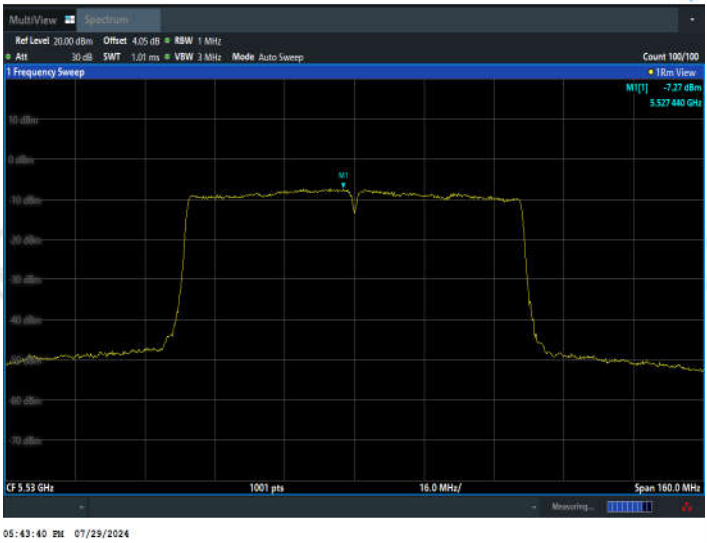
11AC80SISO_Ant2_5530
