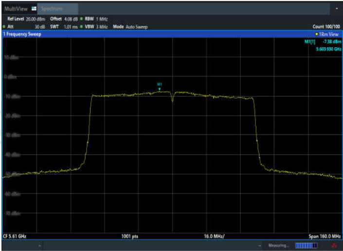
11AC80SISO_Ant2_5610
