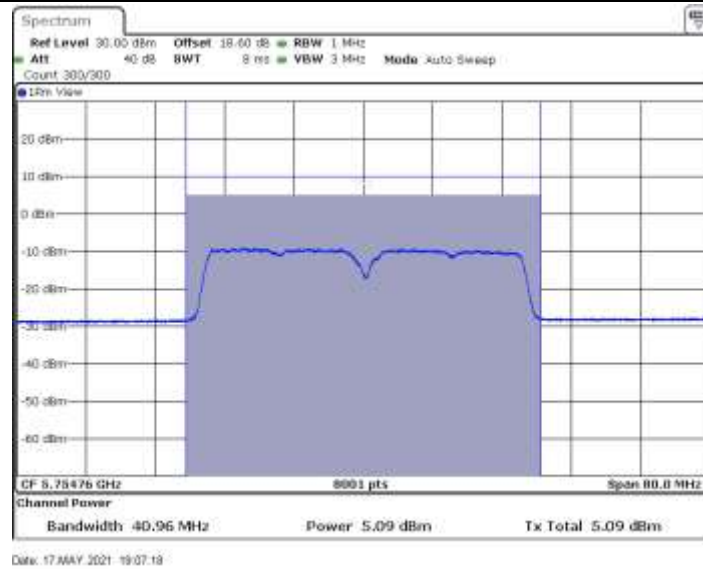
11AC40SISO_Ant2_5755
