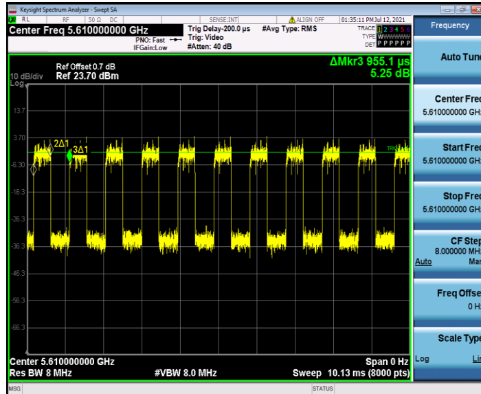
11AC80SISO_Ant2_5610
