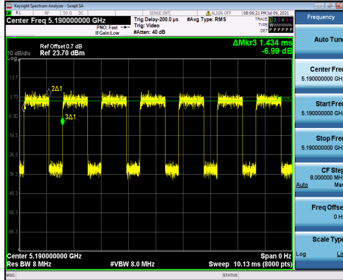
11AC40SISO_Ant2_5190
