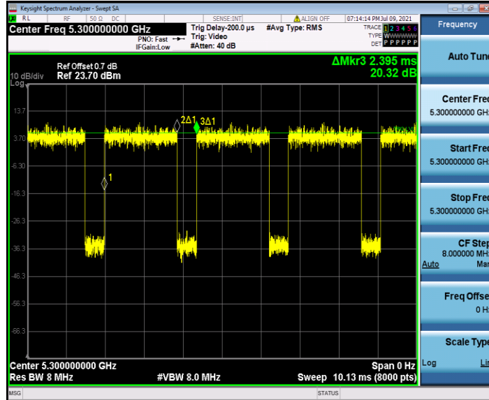
11AC20SISO_Ant2_5300
