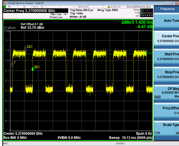
11N40SISO_Ant2_5270
