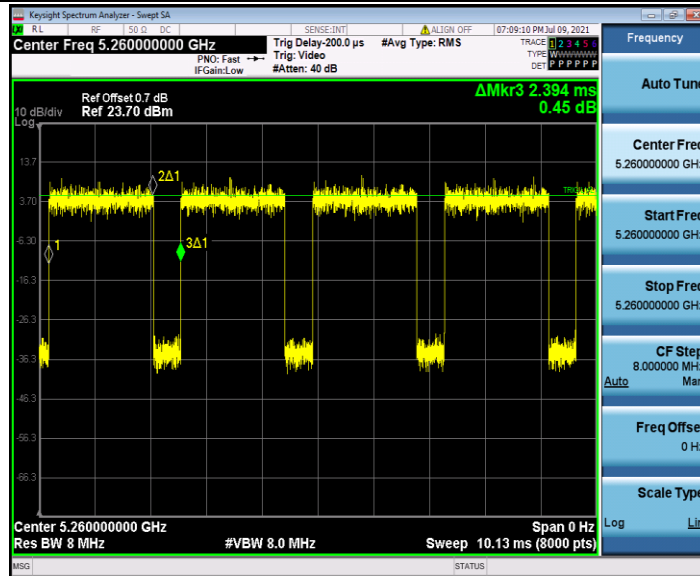
11AC20SISO_Ant2_5260
