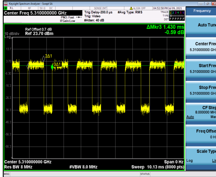
11N40SISO_Ant2_5310
