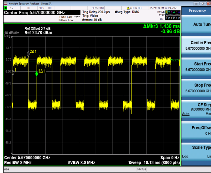
11N40SISO_Ant2_5670
