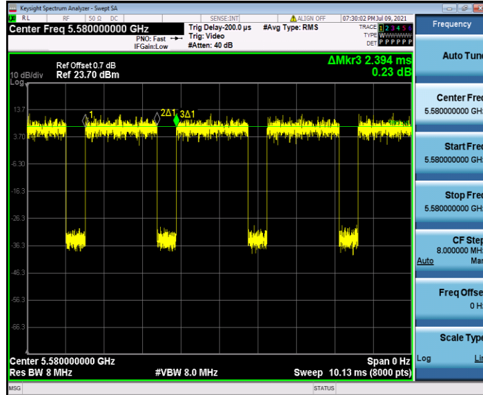
11AC20SISO_Ant2_5580
