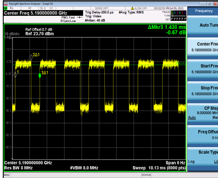
11N40SISO_Ant2_5190
