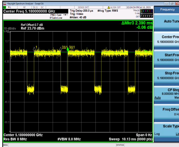
11N20SISO_Ant2_5180
