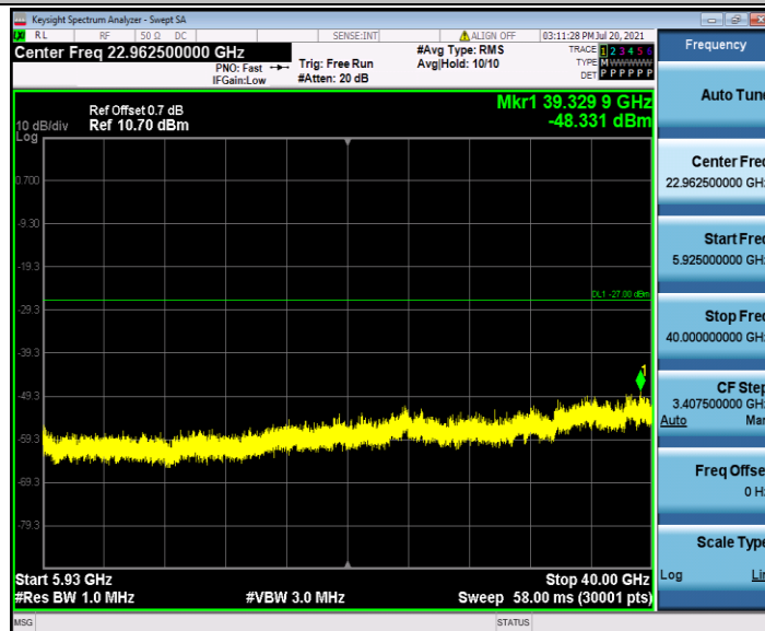
11AC20SISO_Ant2_5785_30~5650
