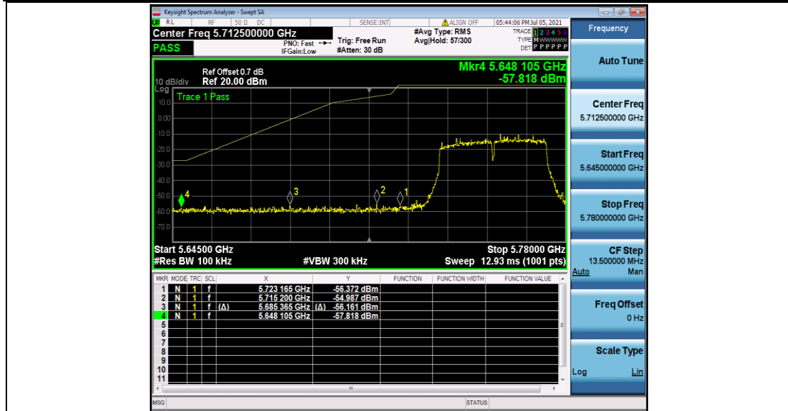
11N40SISO_Ant2_Low_5755
