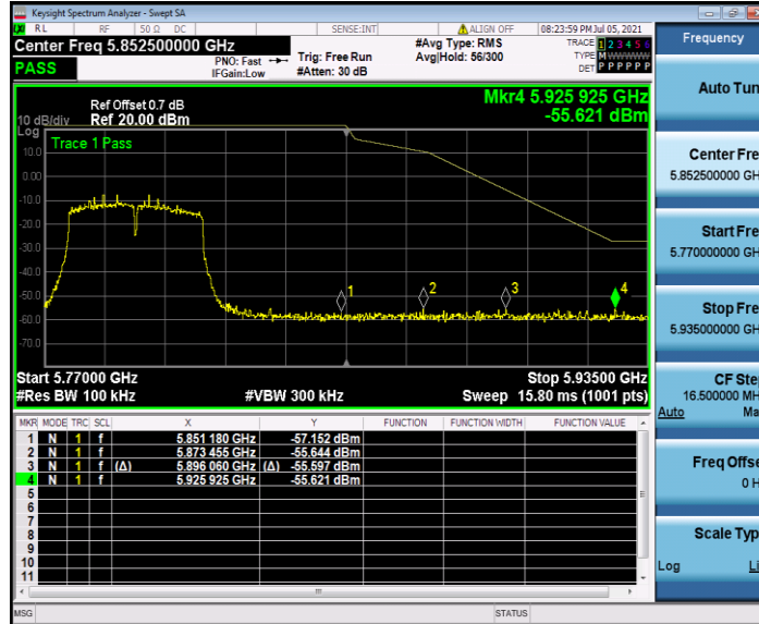
11AC40SISO_Ant2_High_5795
