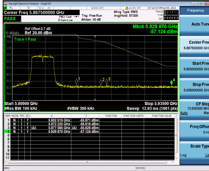
11AC20SISO_Ant2_High_5825
