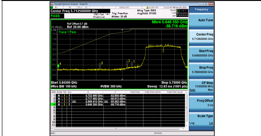
11N40SISO_Ant1_Low_5755
