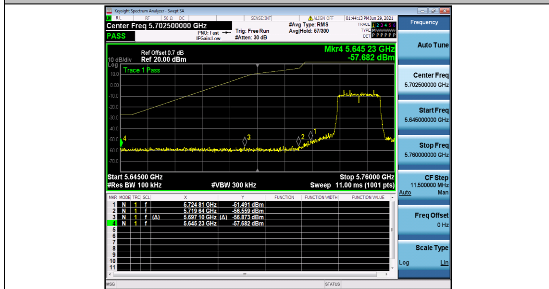
11AC20SISO_Ant2_Low_5745
