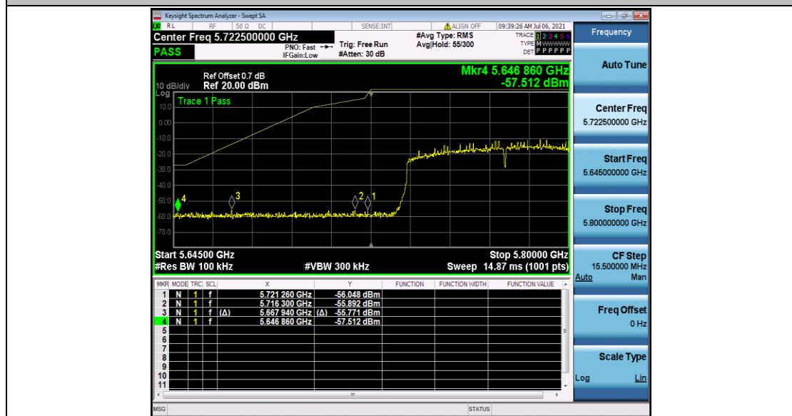
11AC80SISO_Ant2_High_5775
