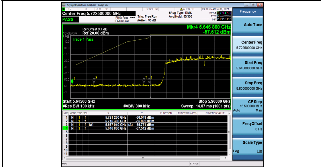
11AC80SISO_Ant2_Low_5775
