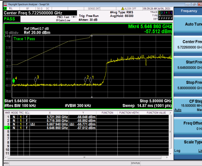
11AC80SISO_Ant2_Low_5775
