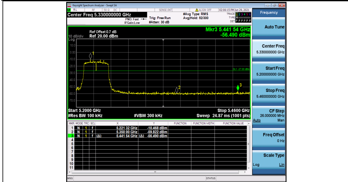
11AC40SISO_Ant2_High_5230
