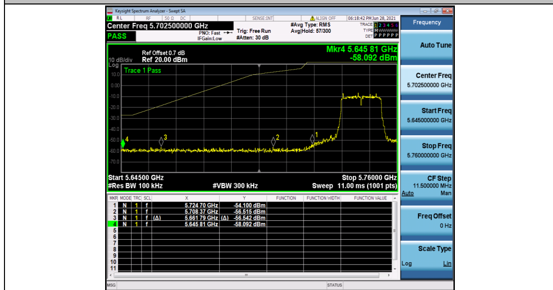
11A_Ant2_Low_5745
