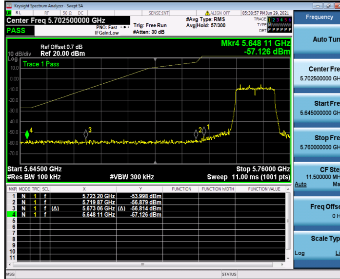
11A_Ant2_Low_5745
