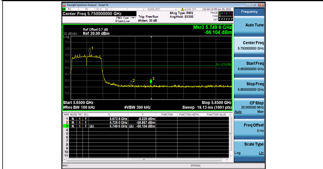
11AC40SISO_Ant2_High_5670
