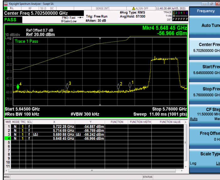
11N20SISO_Ant2_Low_5745
