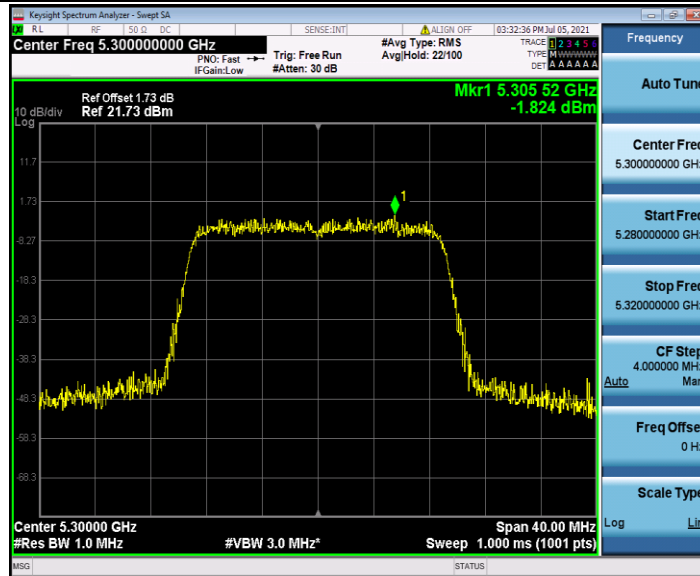
11AC20SISO_Ant2_5300
