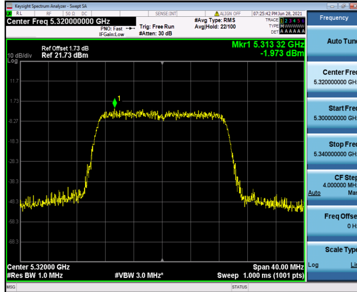
11N20SISO_Ant2_5320
