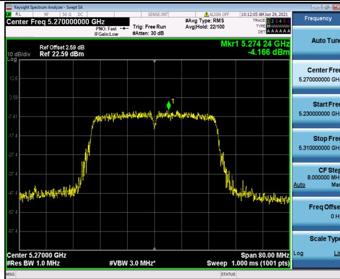
11N40SISO_Ant2_5270
