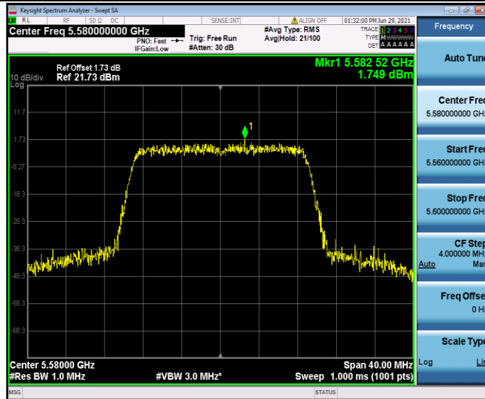
11AC20SISO_Ant2_5580
