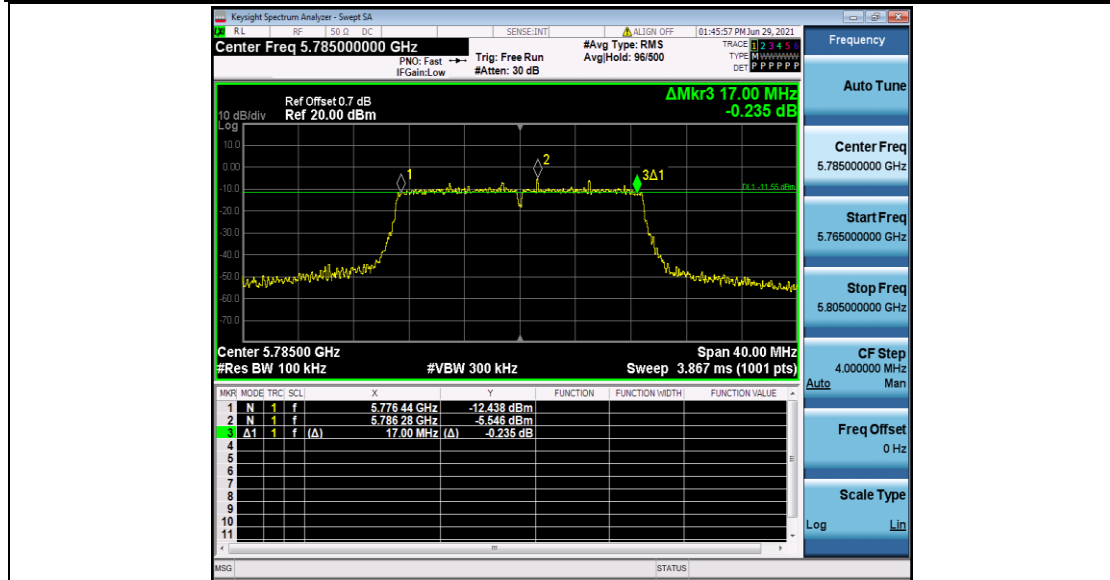
11AC20SISO_Ant2_5785
