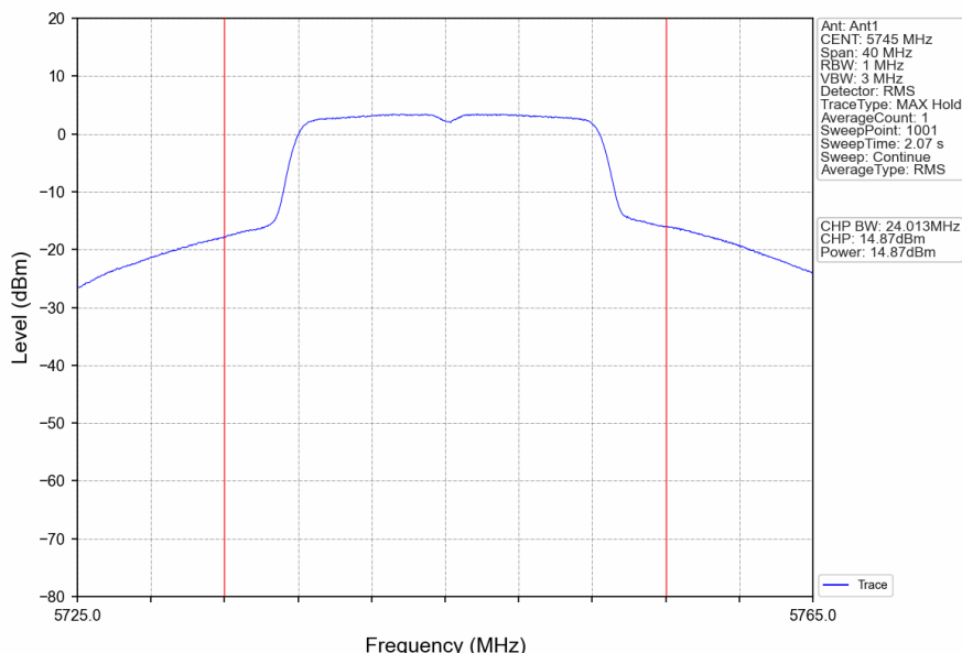
802.11a_LCH_5745MHz_Ant1_NTNV
